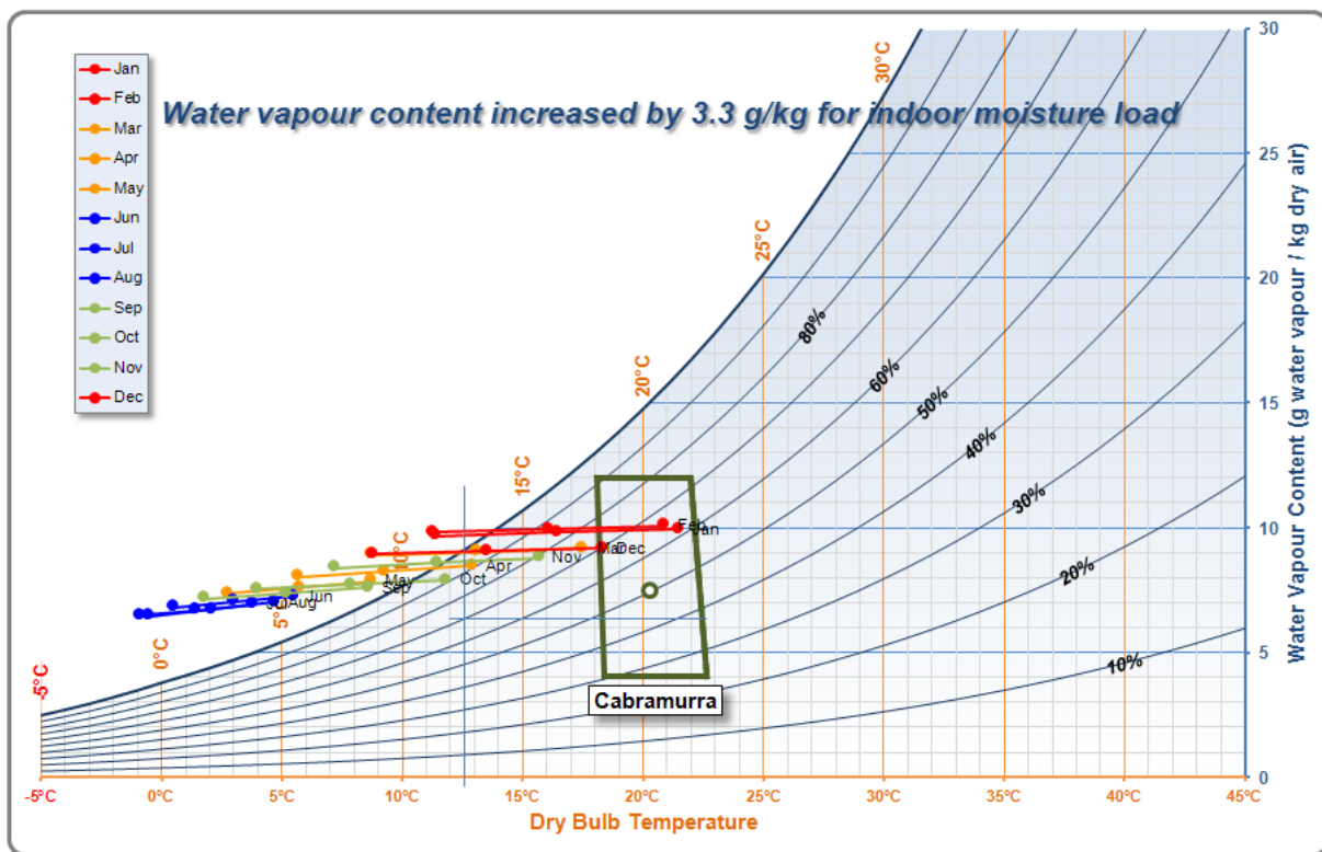
Figure D.13 Water vapour content values adjusted for indoor load – Cabramurra (NSW)
