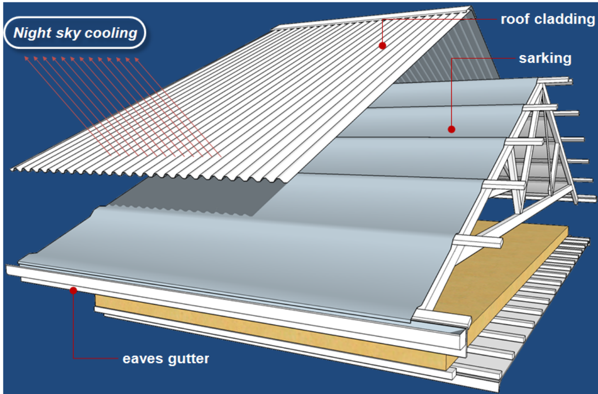
Figure 6.9 Draining condensate formed on the underside of roof cladding
