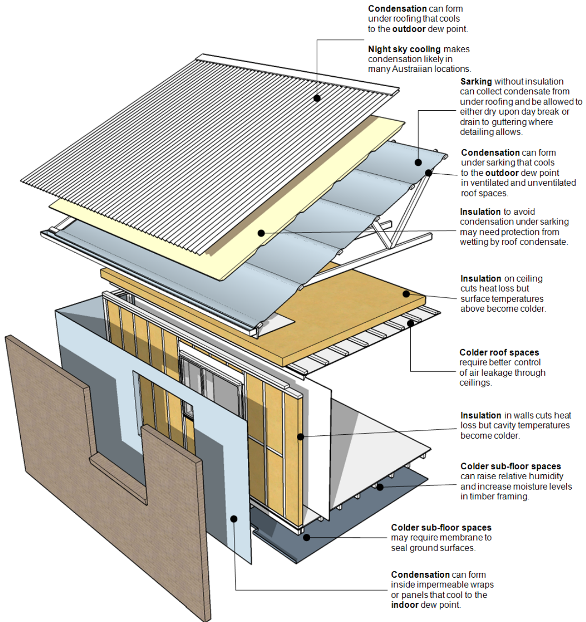
Figure 6.4 Changes to interstitial envelope conditions for a typical masonry veneer house
