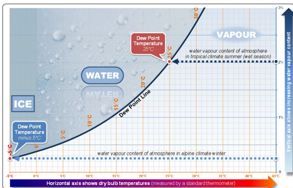
Figure 4.3 Elements of the psychrometric chart
