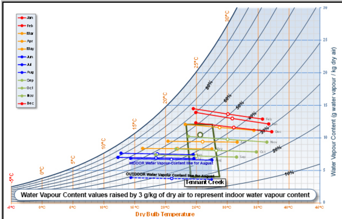
Figure 5.18 Water vapour content values adjusted for indoor load – Tennant Creek (NT)
