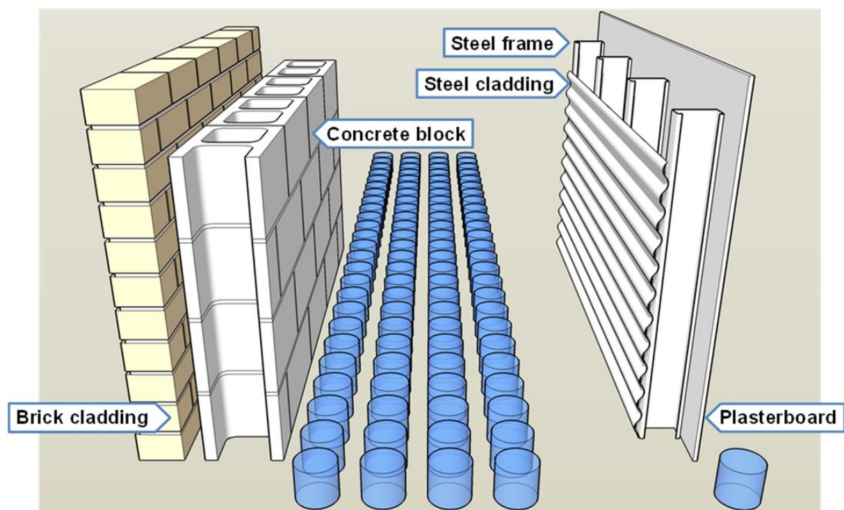
Figure 4.13 Comparative safe moisture storage capacity of masonry and light framed walls
