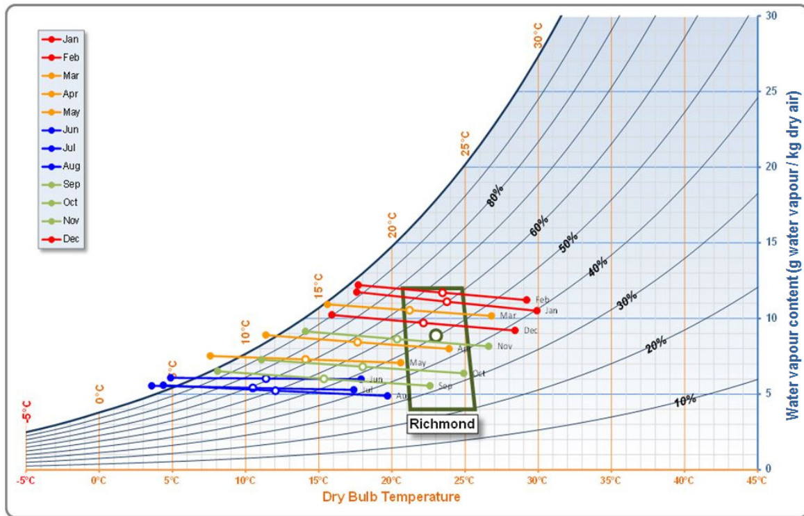
Figure 5.11 Climate analysis on the psychrometric chart: Richmond (NSW) – Mild Temperate
