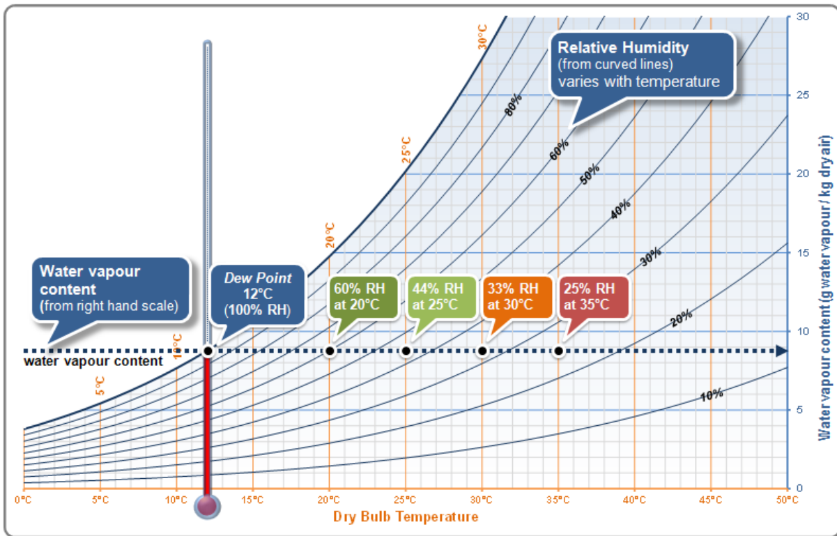
Figure 4.5 Water vapour content and RH on the psychrometric chart
