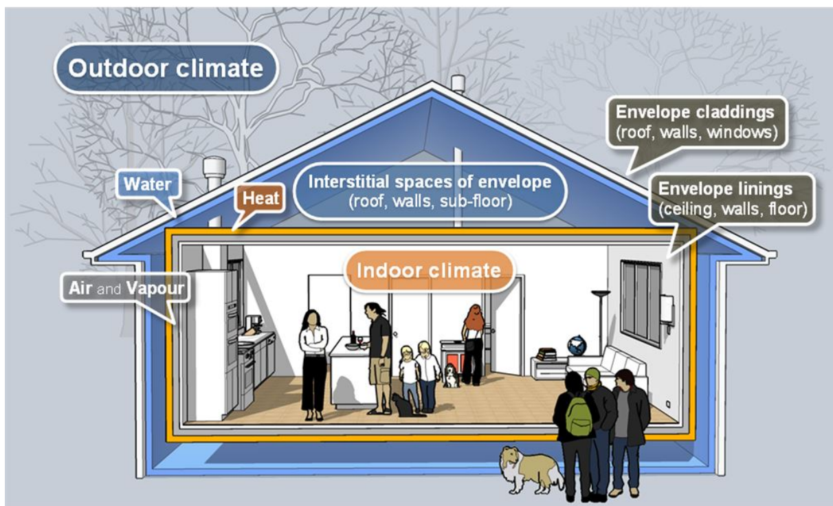
Figure 6.3 Control functions in the interstitial spaces of the building envelope
