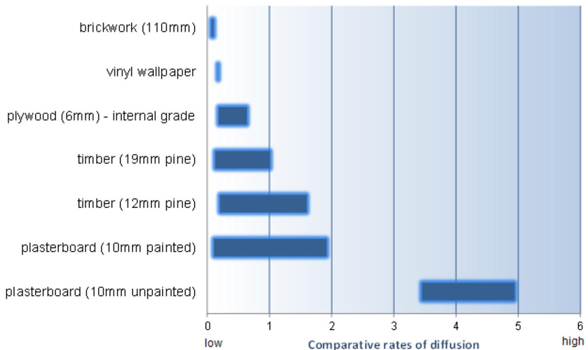
Figure 4.2 Diffusion of water vapour through some permeable building materials (Comparison based on values from BS 5250:2011+A1:2016)
