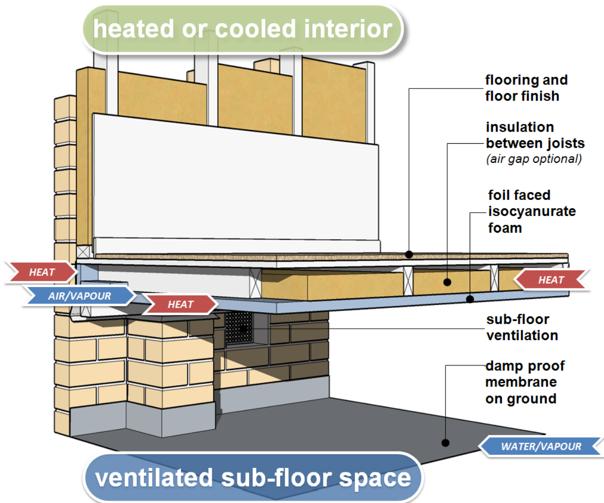
Figure 6.17 Suspended timber framed floor with summertime risk of inward vapour drive
