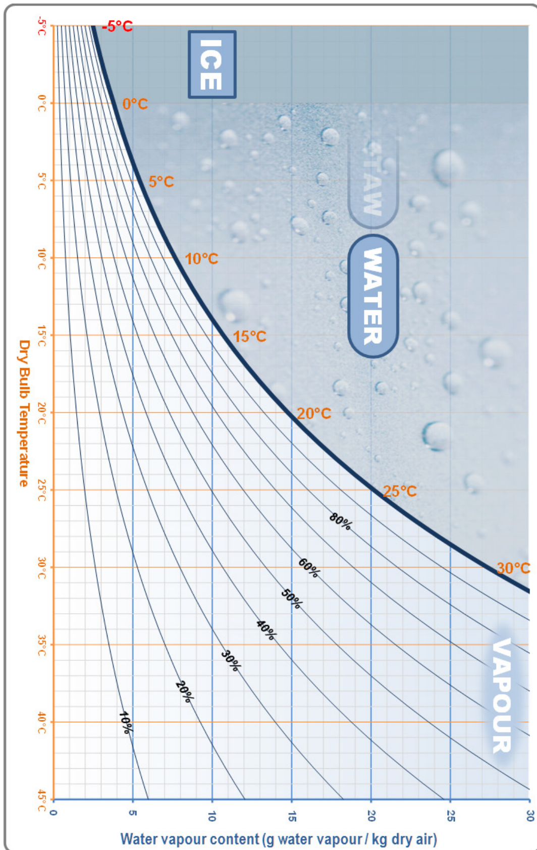
Figure D.14 Basic psychrometric chart for climate analysis
