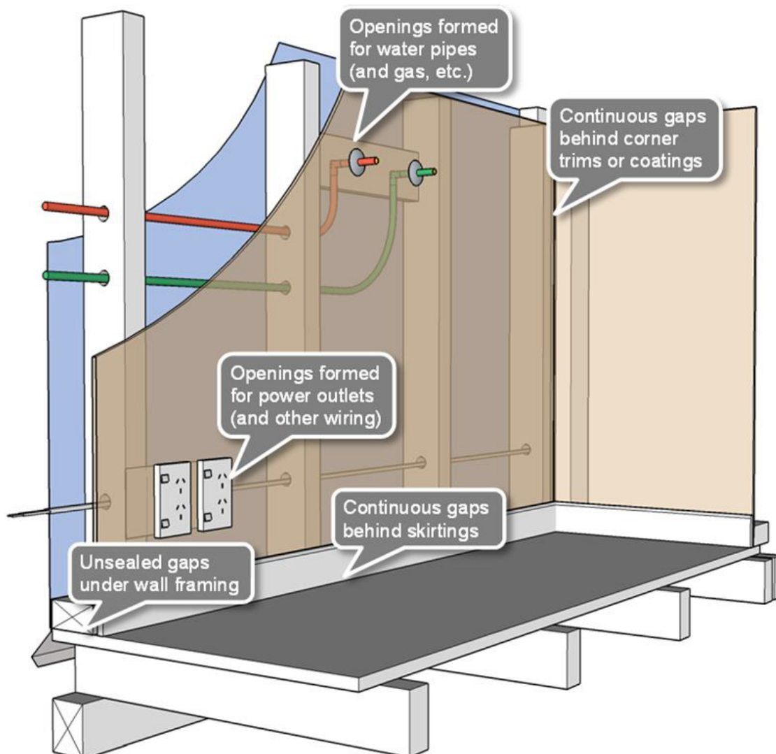
Figure 6.11 Some typical air and water vapour leakage sites through internal wall linings
