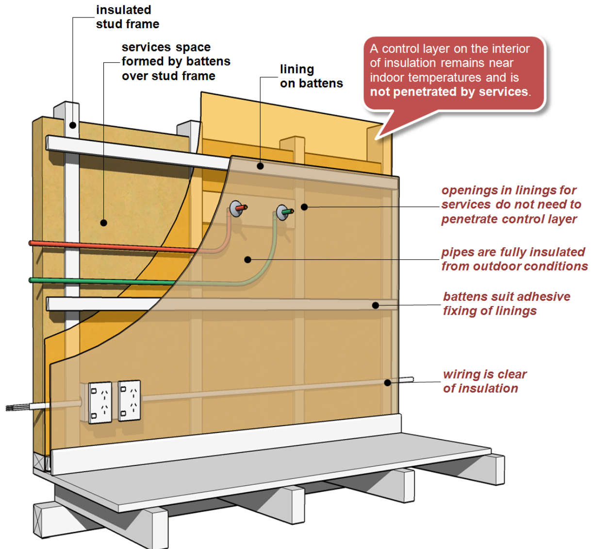
Figure 6.14 Battered services space to avoid penetration of control layers in envelope walls
