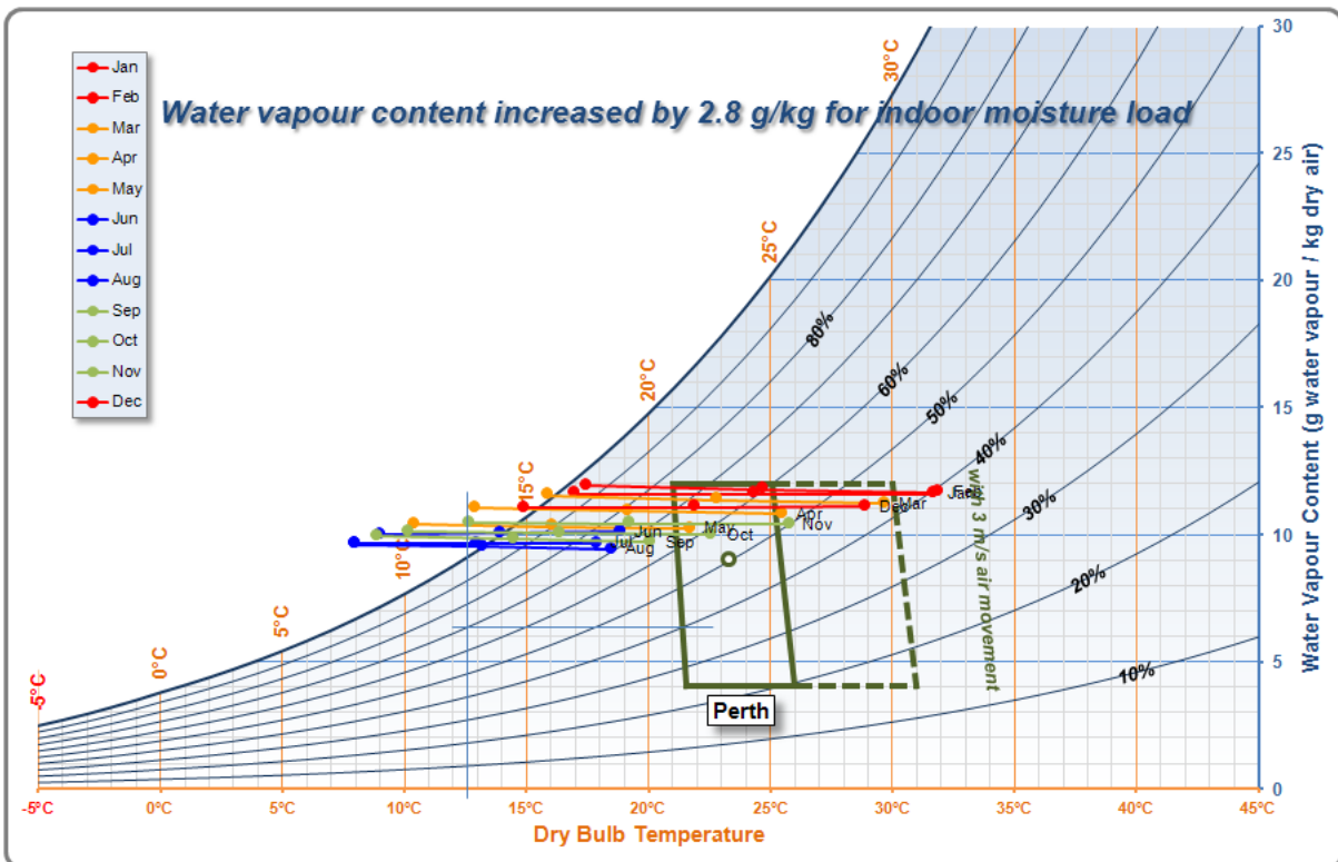
Figure D.7 Water vapour content values adjusted for indoor load – Perth (WA)
