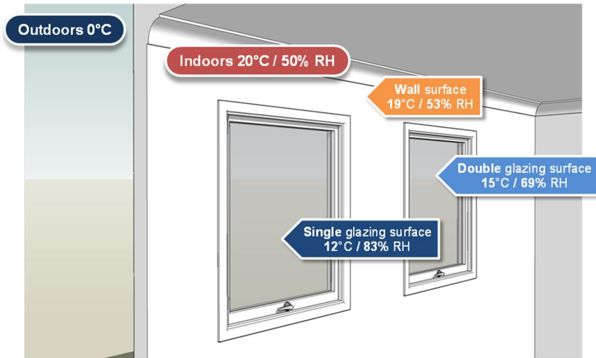
Figure 4.9 Surface temperatures of glazing in interior heated to 20°C (outdoors 0°C)
