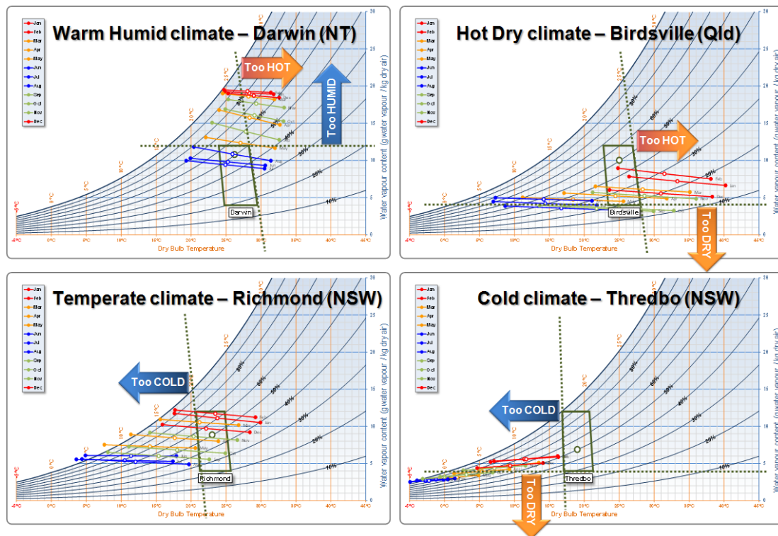
Figure 5.12 Characteristics of the four basic climate types
