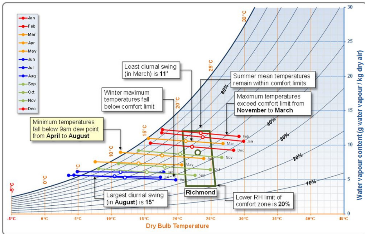
Figure 5.13 Annotated climate analysis for Richmond (NSW) – Mild Temperate
