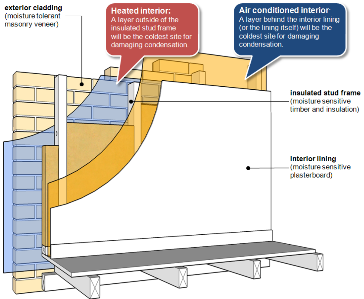
Figure 6.7 Critical condensation surfaces in masonry veneer envelope walls
