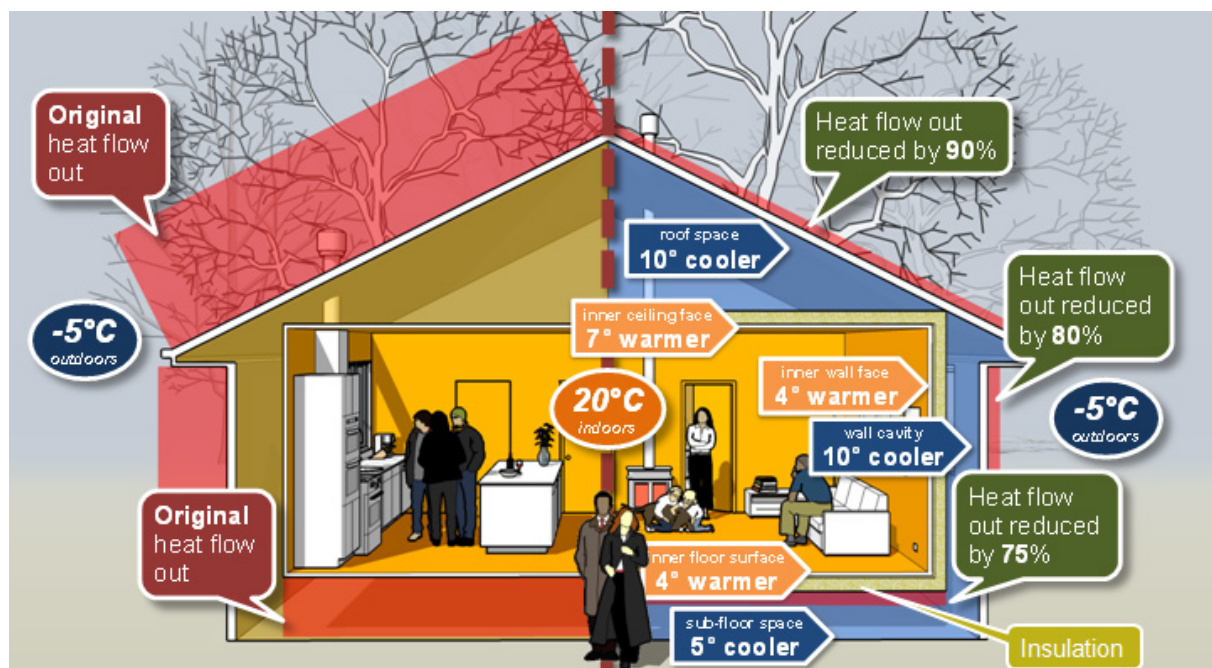
Figure 3.5 Heat loss and temperature change effects of NCC energy efficiency provisions for a home (All added insulation is placed on the ceiling, in wall frame or under flooring)
