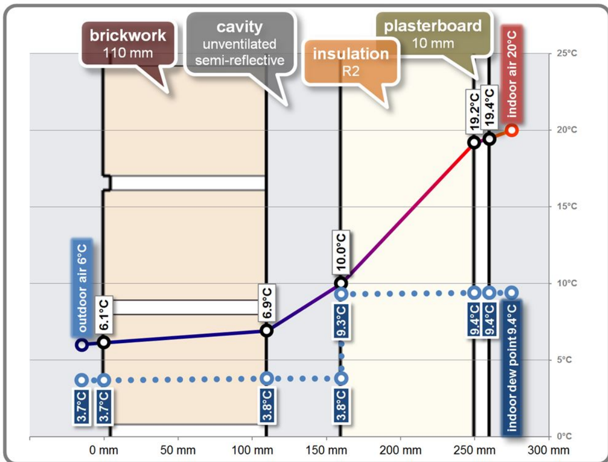
Figure 6.19 Steady state comparison of temperature and dew point gradients across a wall (Note: the assumption of a wall wrap with an exterior anti-glare coating provides the semi-reflective cavity indicated in the figure below)
