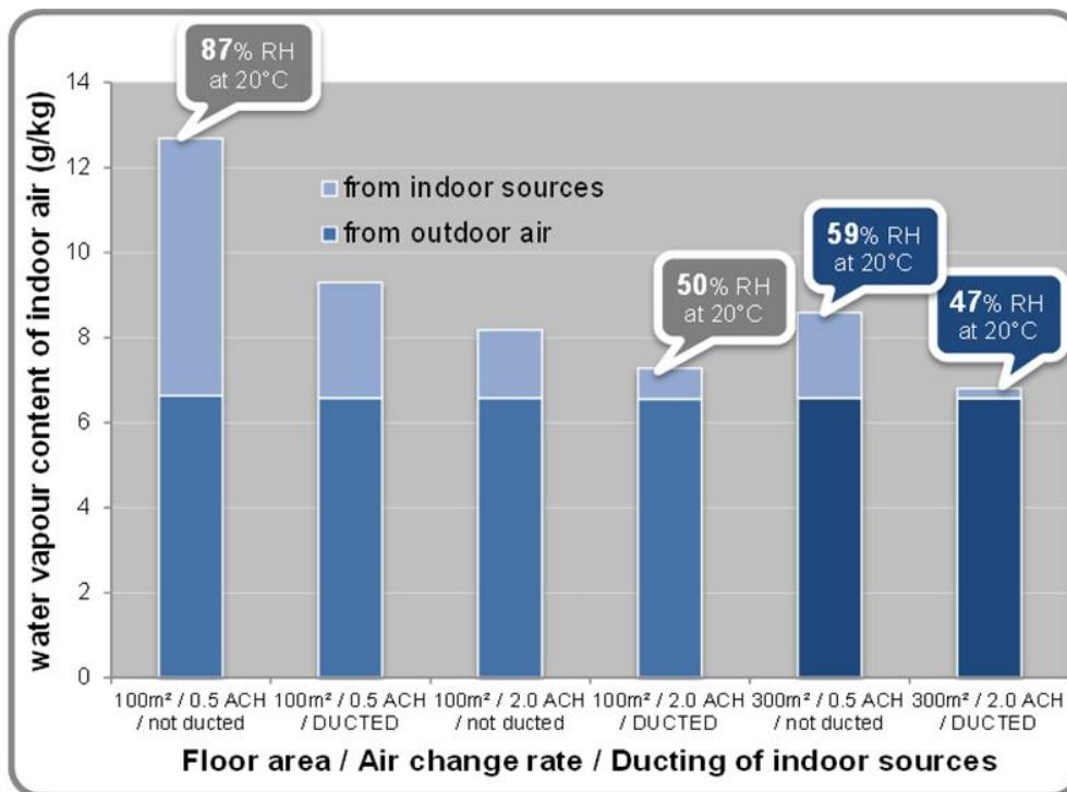
Figure 5.15 Impact of indoor volume, air change rate and ducting of sources on indoor humidity
