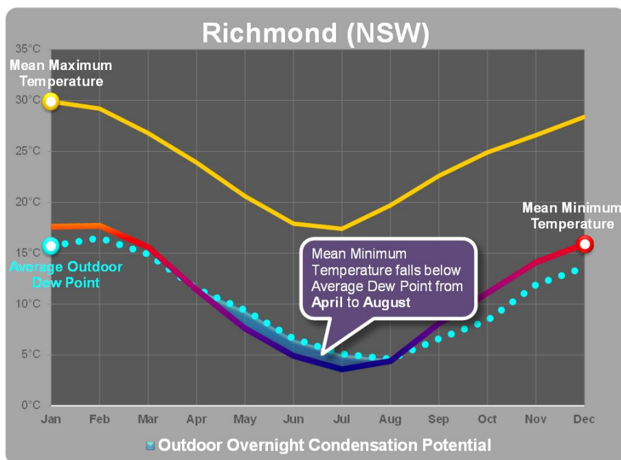
Figure 5.7 Comparison of monthly mean minimum temperatures and average dew points (outdoor overnight condensation potential)
