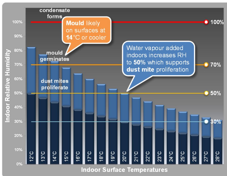
Figure 4.7 Warmer indoor temperature lowering RH of outdoor air from outdoors
