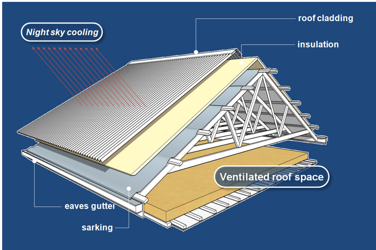
Figure 6.18 Minimising condensation on the underside of sarking - sarking as temperature control
