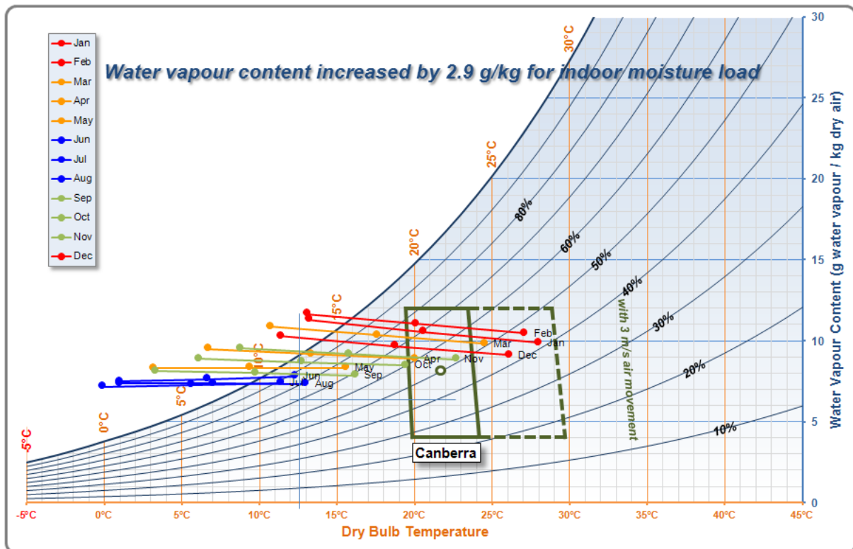
Figure D.11 Water vapour content values adjusted for indoor load – Canberra (ACT)
