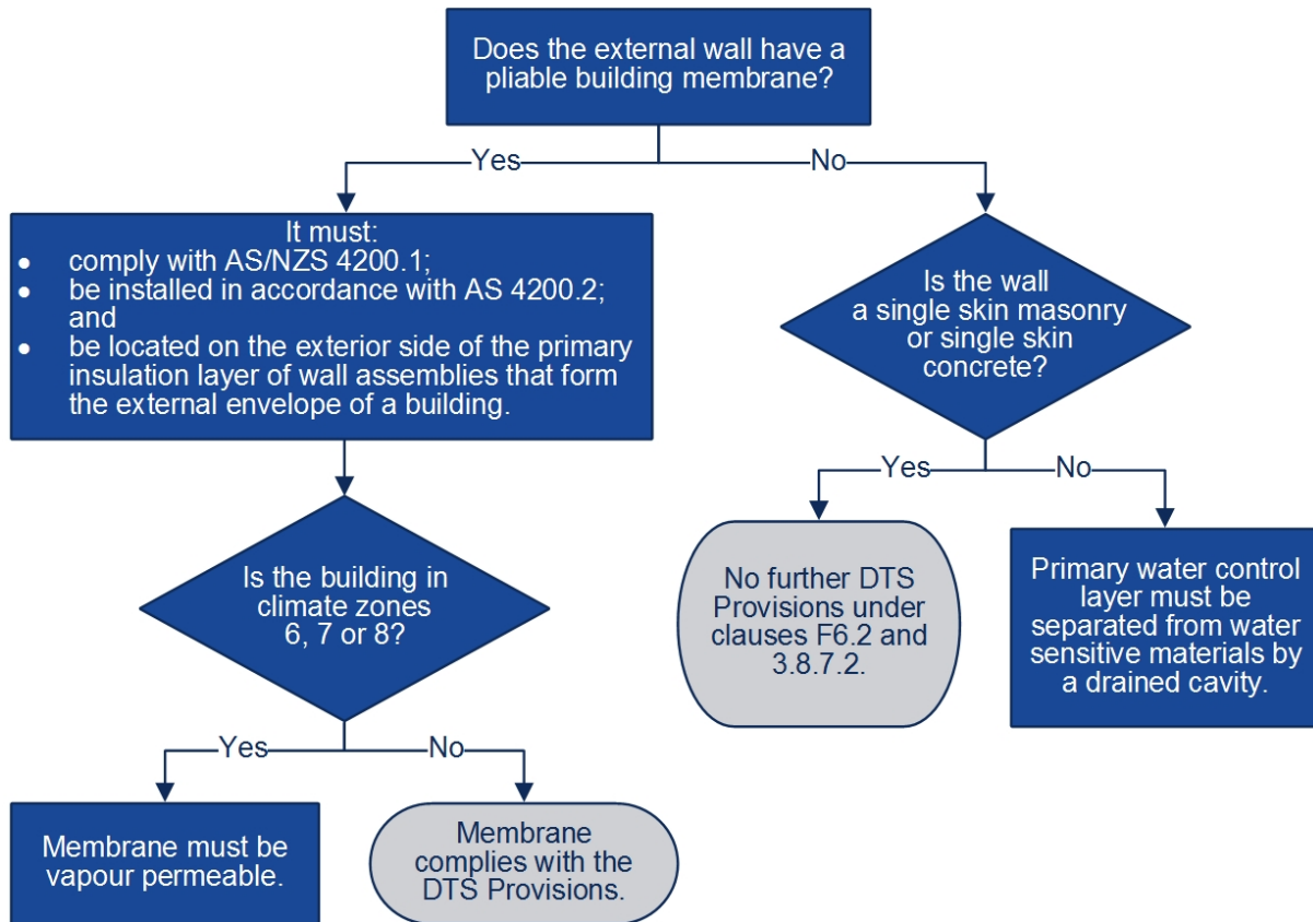
Figure 7.2 Simplified flowchart for pliable building membranes (refer to F2.6 and 3.8.7.2 in NCC Volume One and Two respectively)
