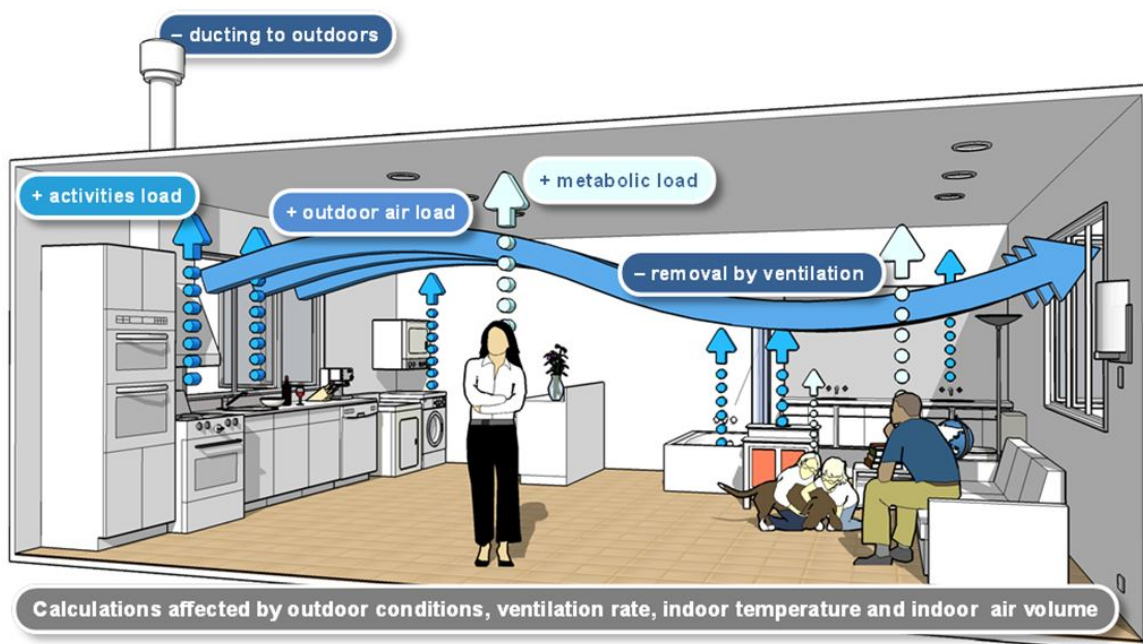
Figure 5.14 Factors affecting daily average indoor water vapour levels
