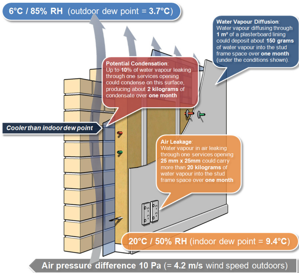
Figure 6.13 Comparison of water vapour transport by diffusion and by air leakage
