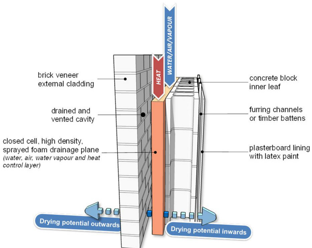
Figure 6.15 Joseph Lstiburek’s ‘Clever Wall’ - using a single material for four control functions (Source: Lstiburek 2010, Figure 7) (Note: Latex paint is a water based paint)
