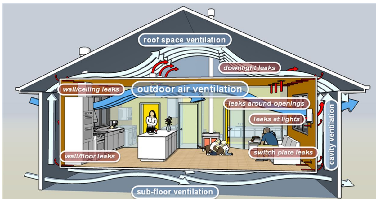
Figure 3.1 Air and water vapour movement through the building interior and the building fabric
