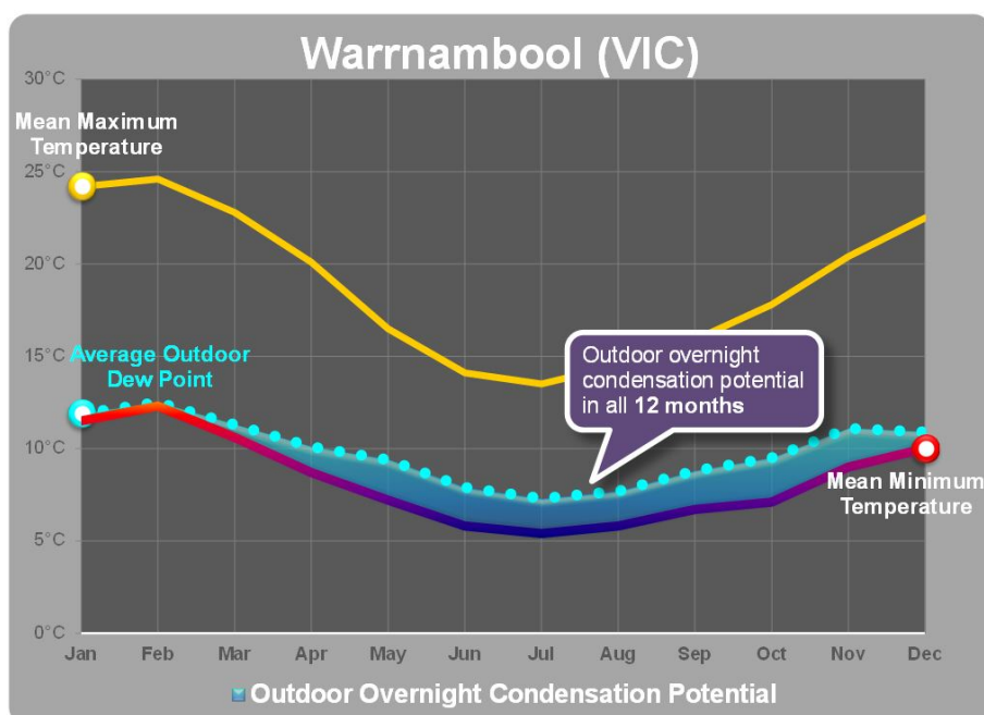
Figure 5.8 Outdoor overnight condensation potential spanning all 12 months
