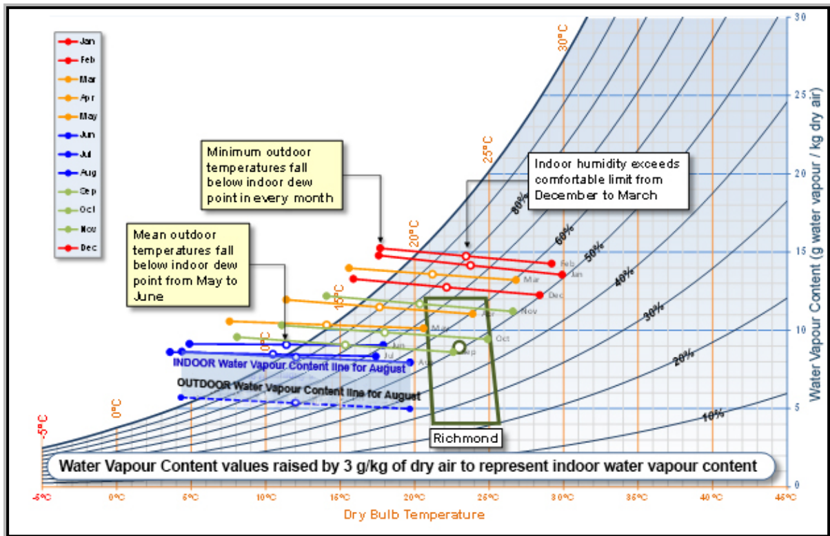
Figure 5.17 – Water vapour content values adjusted for indoor load – Richmond (NSW)
