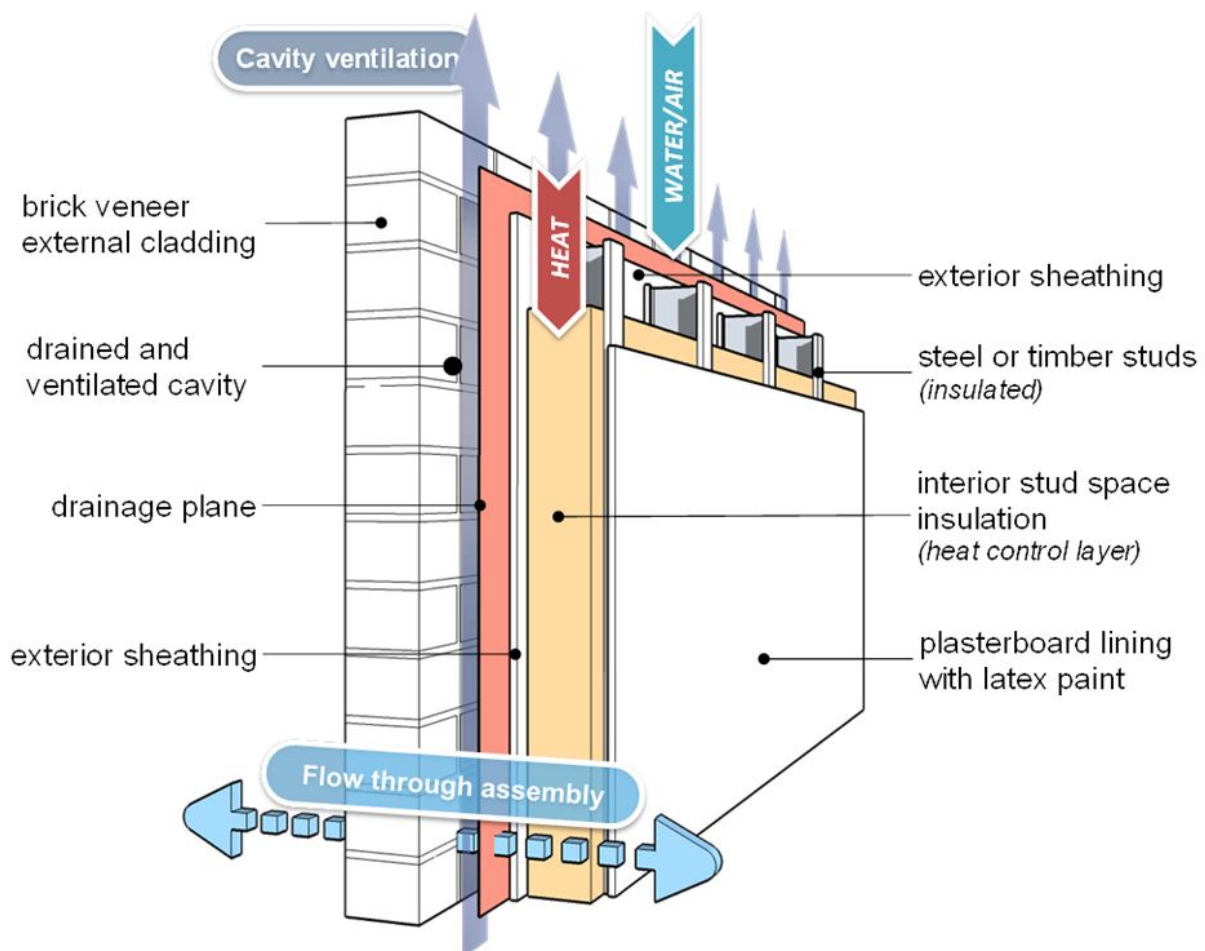
Figure 6.16 Insulated stud frame wall with brick veneer cladding (Source: Lstiburek 2011b, Figure 6) (Note: Latex paint is a water based paint)
