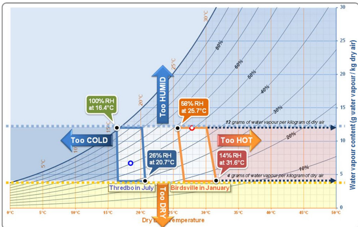
Figure 5.10 Range of human comfort limits for Australian climates (outdoors)
