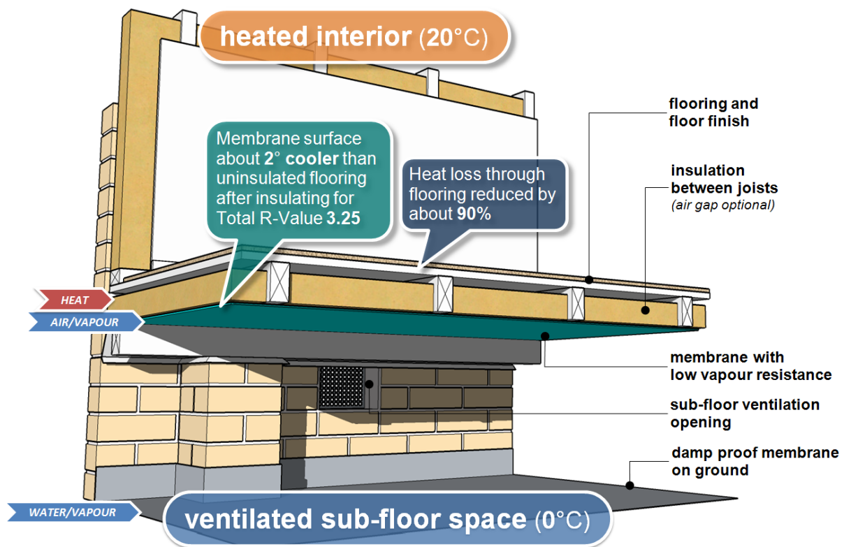
Figure 6.5 Suspended timber framed floor - insulated between joists (alpine/cold climate)
