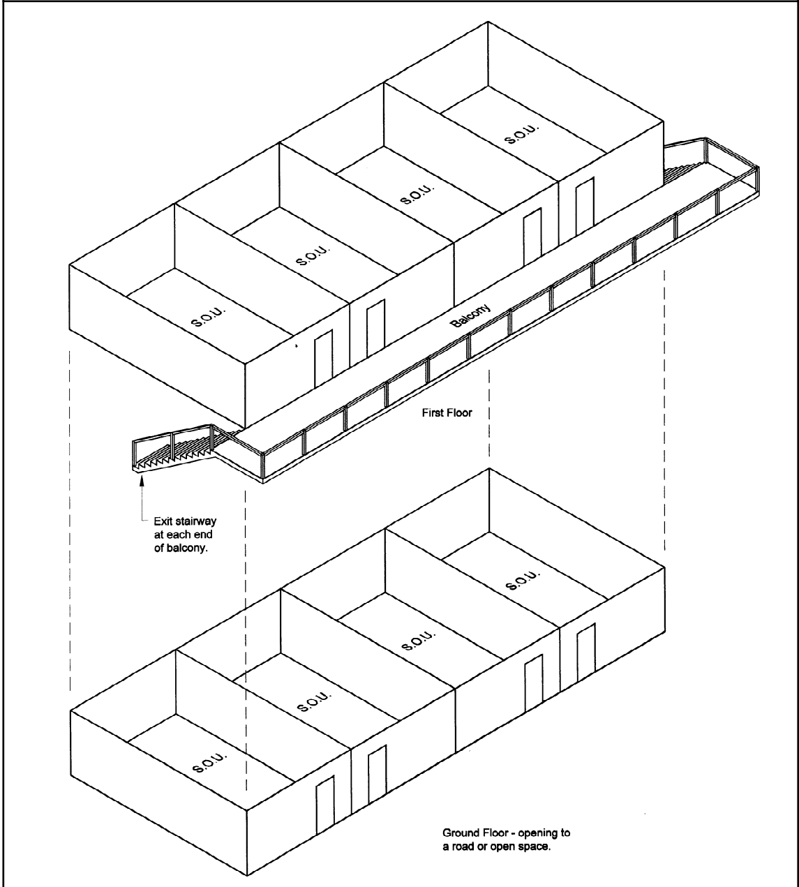
Figure C1.5 EXAMPLE OF THE CONCESSION ALLOWED BY C1.5
