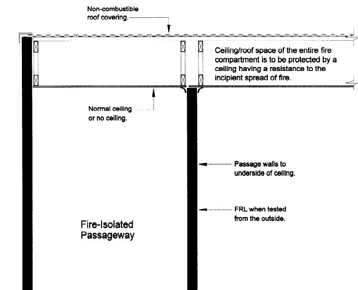
Fire-Isolated Passageway Figure D2.11
