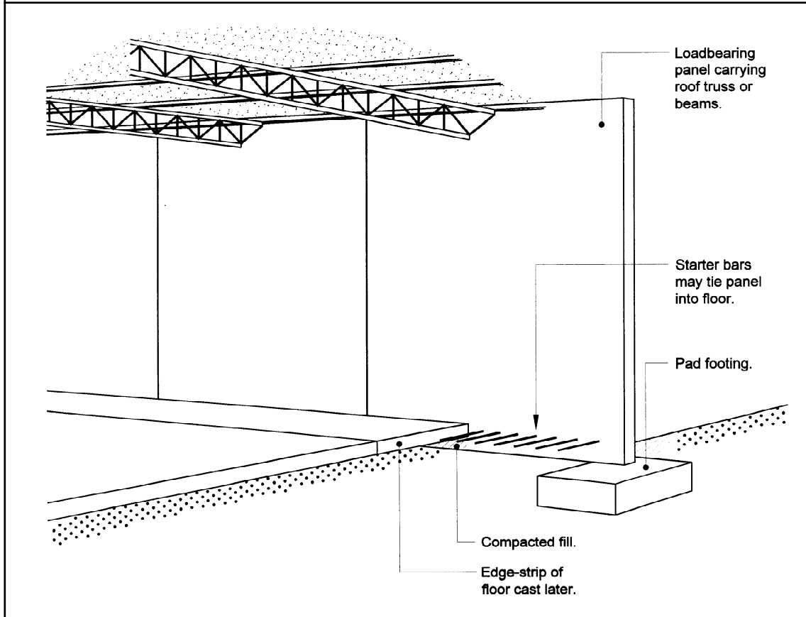
Figure Spec C1.11(2) TYPICAL LOADBEARING PANELS REQUIRED TO COMPLY WITH SPECIFICATION C1.11
