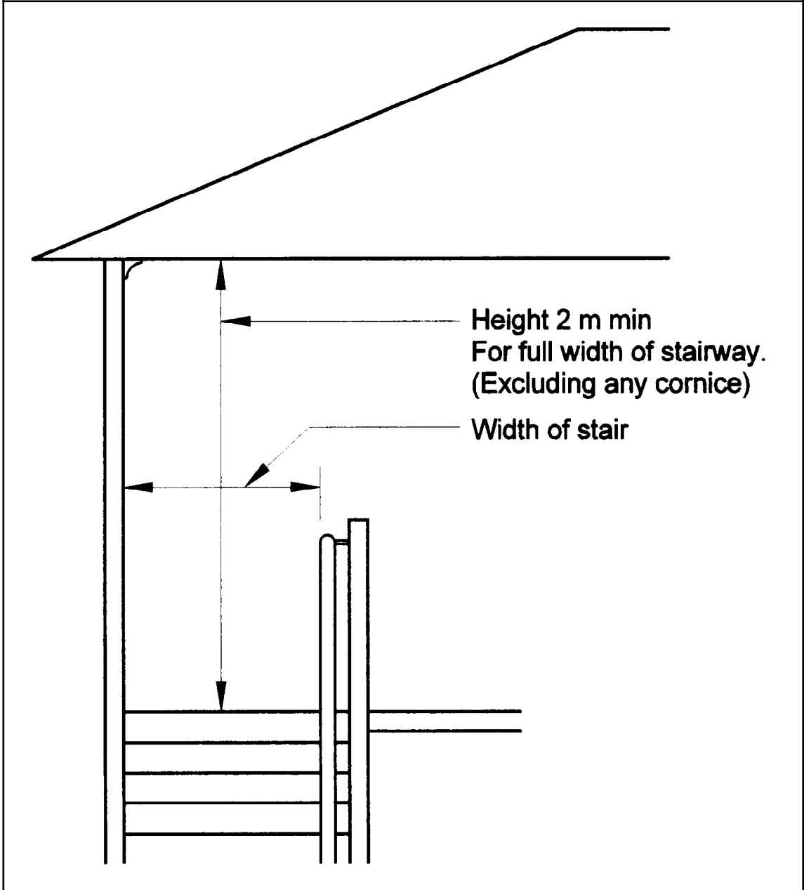
Figure D2.9 METHOD OF MEASURING HEIGHT AND WIDTH OF A STAIRWAY
