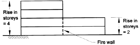
(b) Considered as two separate buildings
