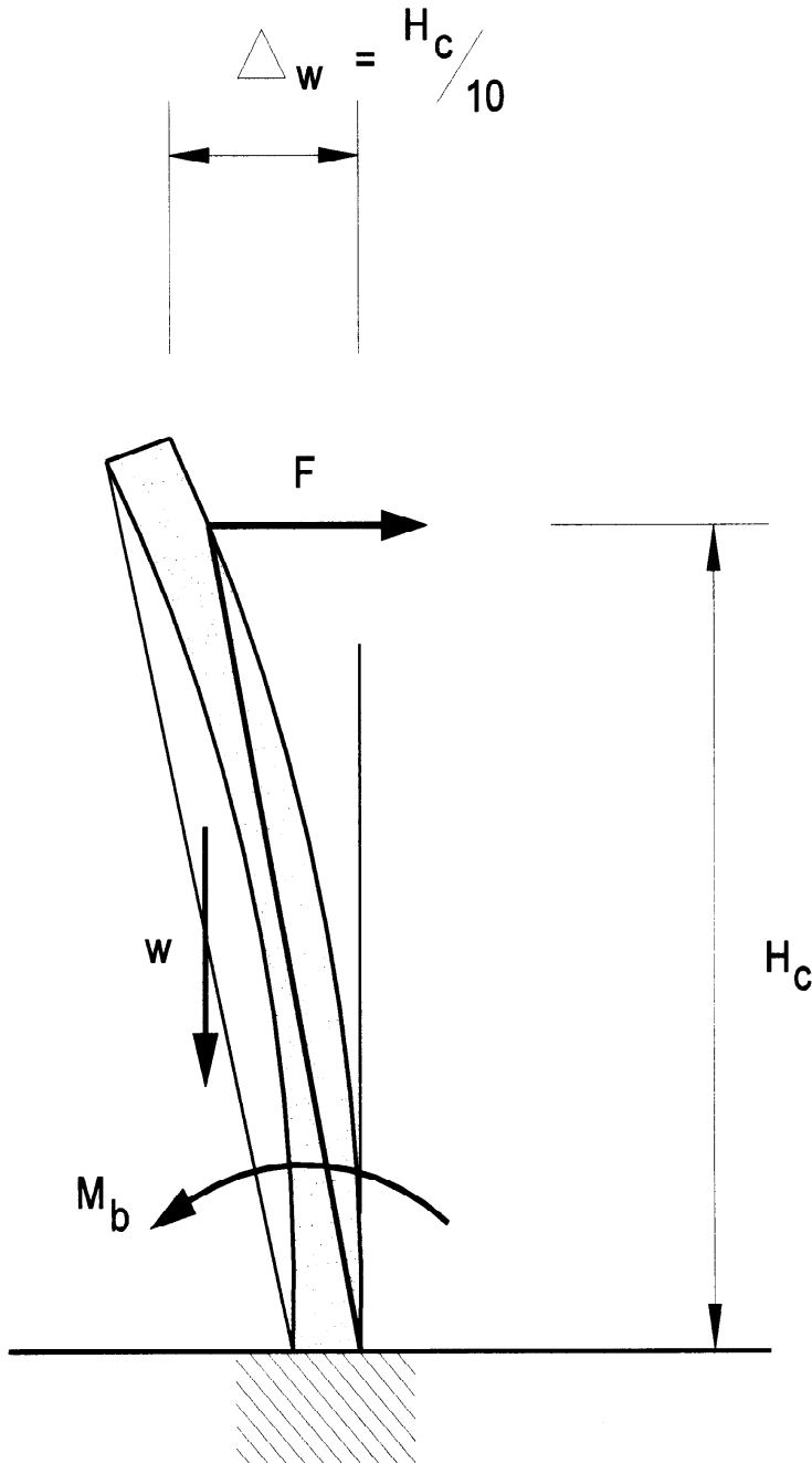
Figure C1.11(4) FORCES TO PULL PANEL INWARDS
