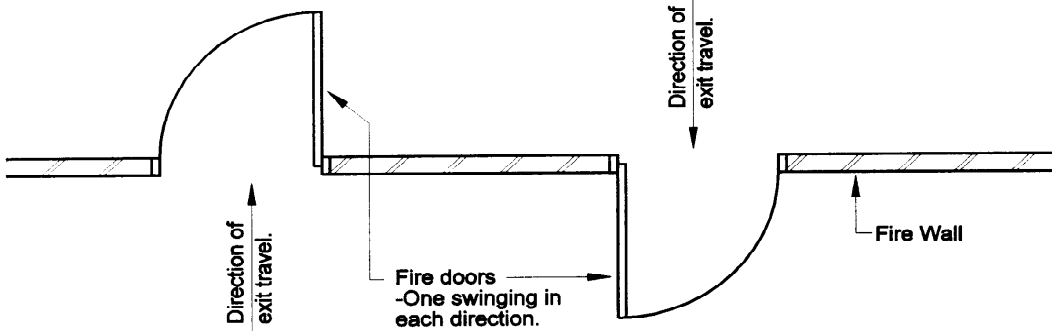
Figure C3.7 PLAN SHOWING HORIZONTAL EXITS IN A FIRE WALL
