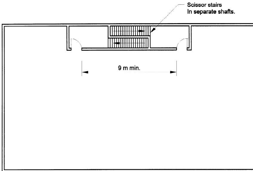
Figure D1.5(2) illustrates the convergence prohibition on alternative paths of travel.
