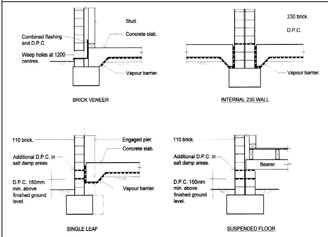
Figure F1.10 INSTALLATION OF DPC IN SUB-FLOOR STRUCTURES
