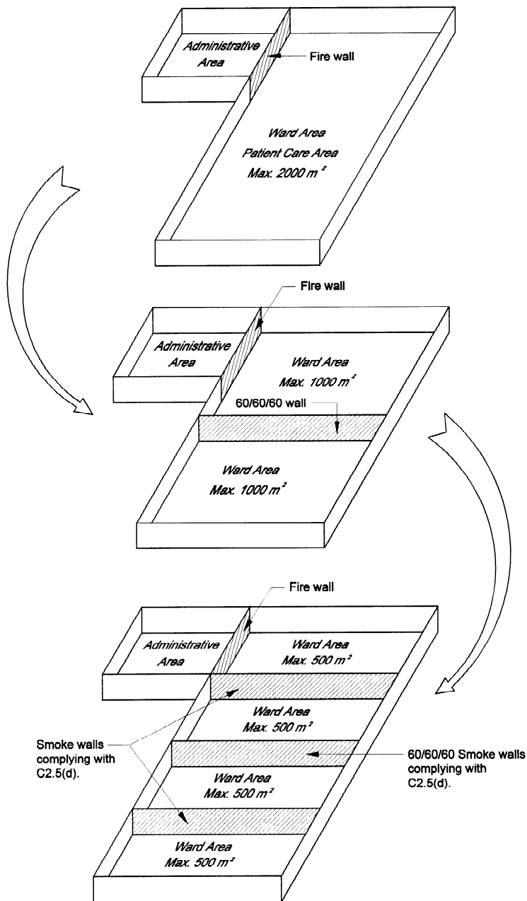
Figure C2.5 PLAN SHOWING ONE METHOD OF COMPLYING WITH C2.5(a) FOR CLASS 9a BUILDINGS
