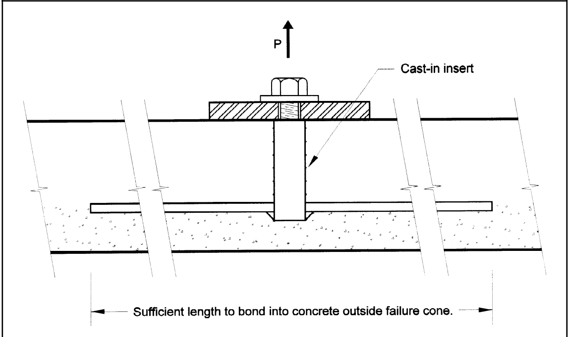
Figure Spec C1.11(3) TYPICAL ANCHOR BARS FOR INSERTS
