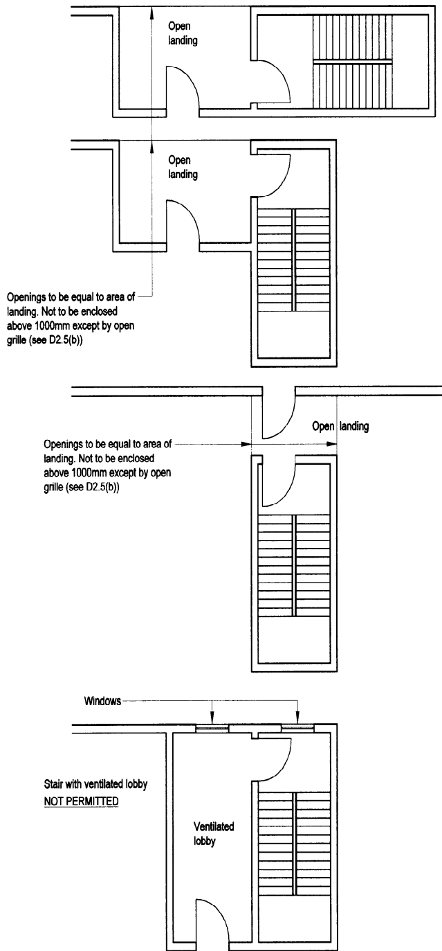
Figure D2.5 PLAN SHOWING COMPLIANCE AND NON-COMPLIANCE WITH D2.5
