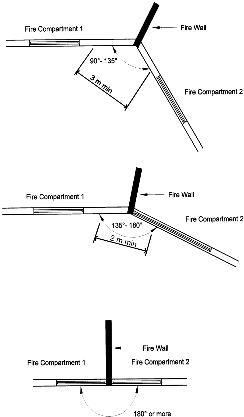
Figure C3.3 PLAN SHOWING ILLUSTRATION OF TABLE C3.3
