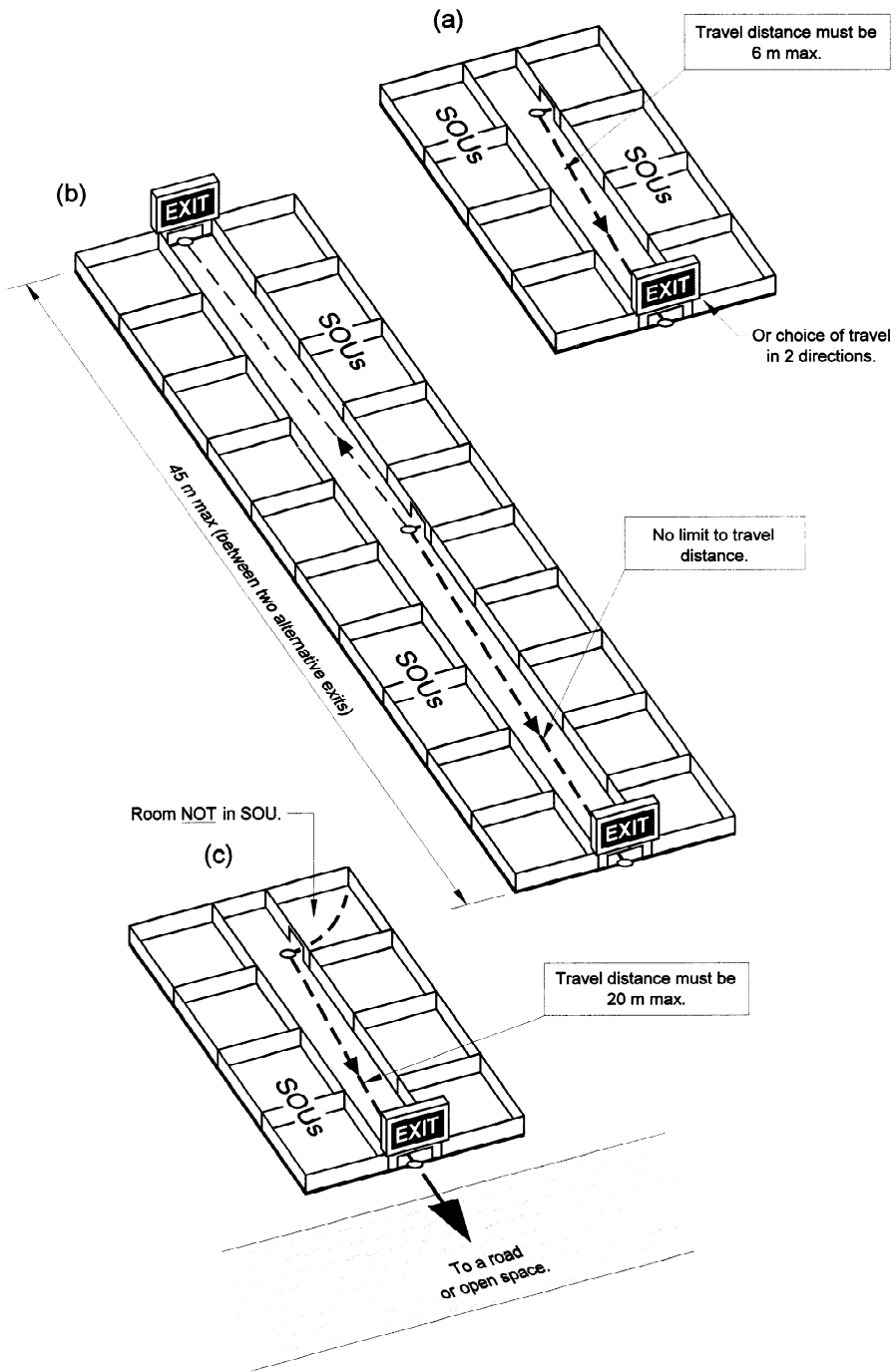
Figure D1.4(1) DISTANCES TO EXITS IN CLASS 2 AND CLASS 3 BUILDINGS
