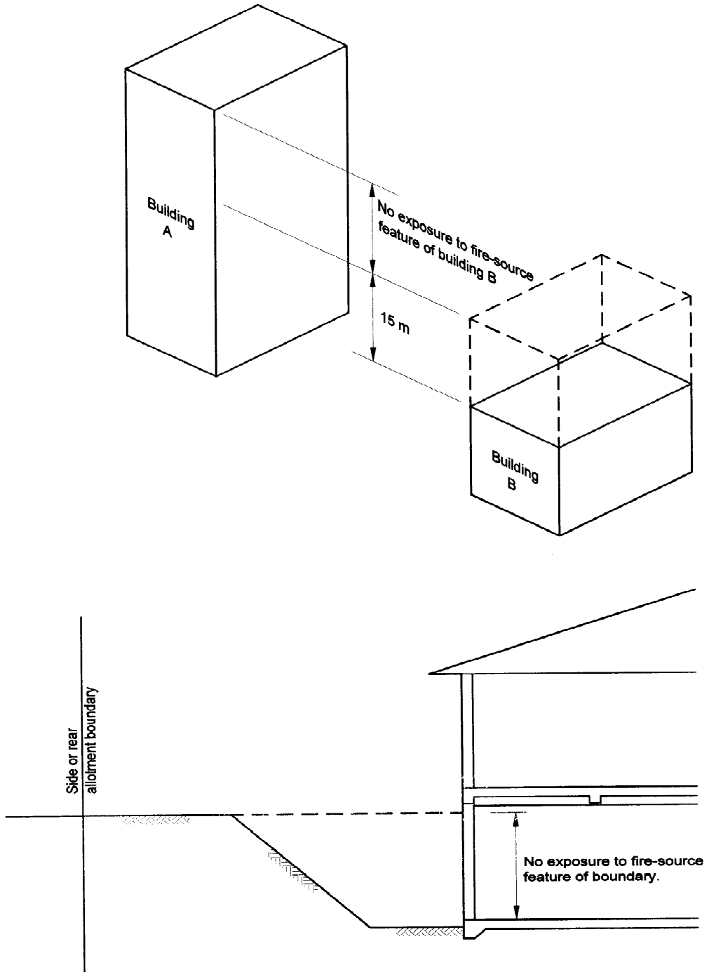
Figure Spec C1.1(1) PART OF A BUILDING NOT EXPOSED TO A FIRE-SOURCE FEATURE
