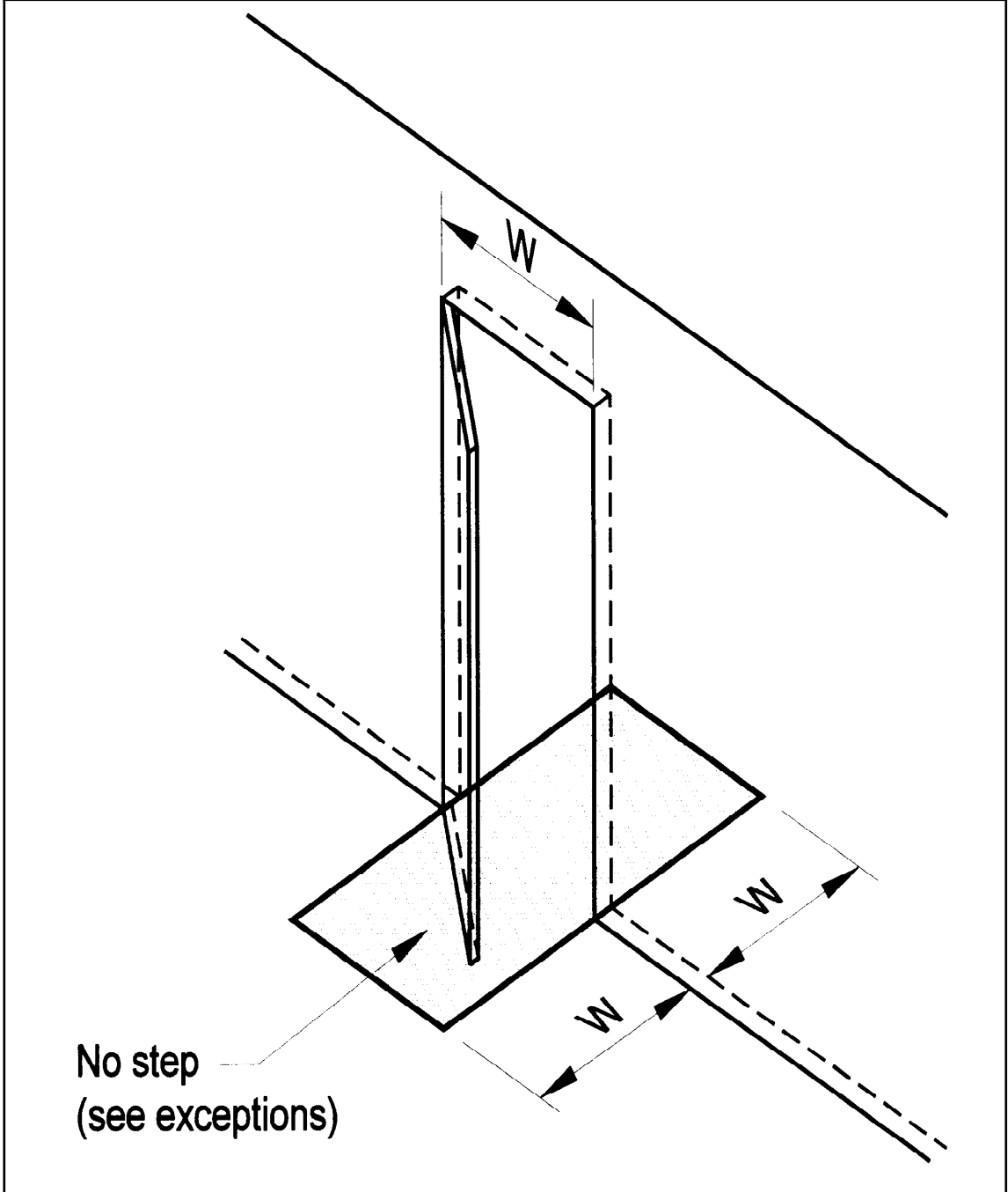
Figure D2.15(1) ILLUSTRATION OF WHERE A STEP IS NOT ALLOWED IN A DOORWAY
