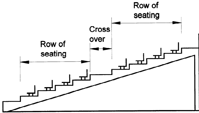
One tier of seating
