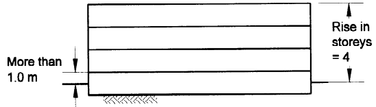
(d) Storey below ground included in calculation of rise in storeys
