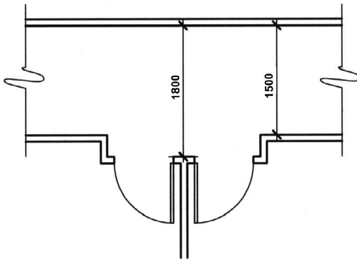
Plan View Example Two
