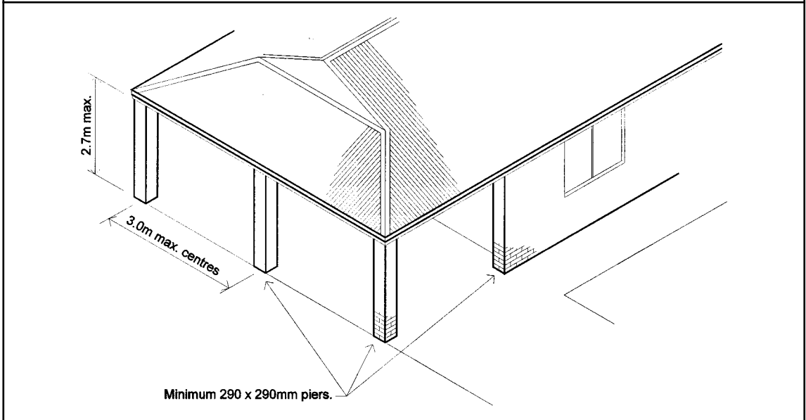
Figure 3.3.1.6 SUB-FLOOR ISOLATED PIERS—MAXIMUM HEIGHTS
