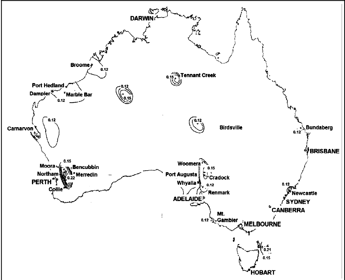
Figure 3.10.2.1 ACCELERATION CO-EFFICIENT MAP OF AUSTRALIA
