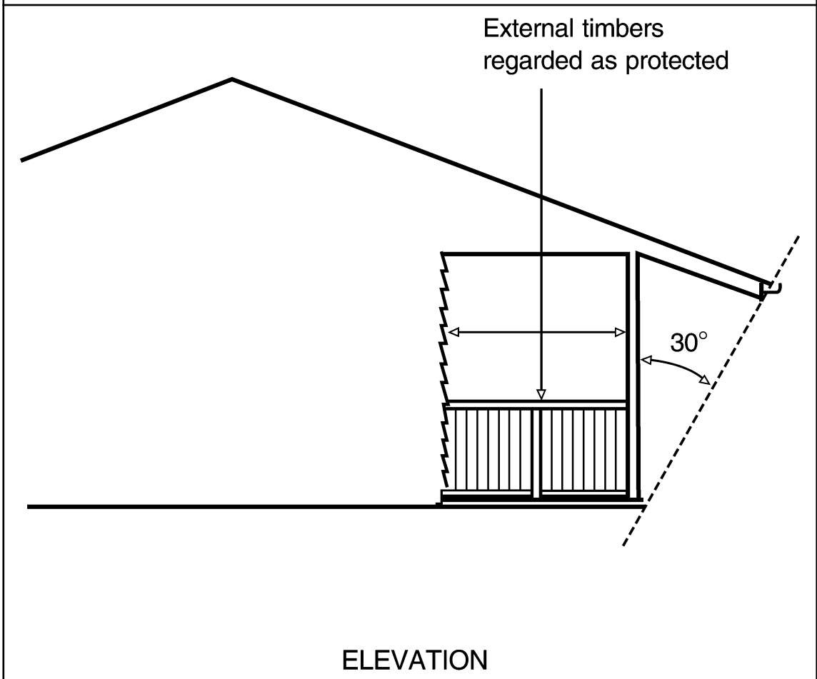
Figure 3.7.4.5 EXTERNAL TIMBERS REGARDED AS PROTECTED
