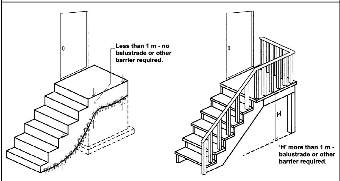
Figure 3.9.2.3 BALUSTRADES OR OTHER BARRIERS—WHEN REQUIRED
