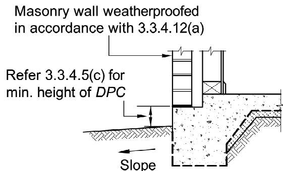
(e) Weatherproofed masonry veneer
