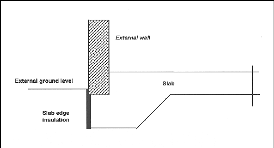
Figure 3.12.1.5 INSULATION OF SLAB EDGE
