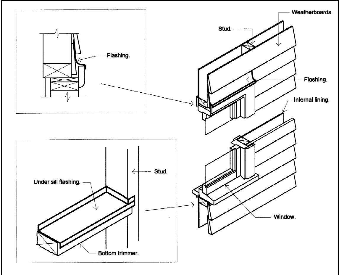
Figure 3.5.3.4 TYPICAL WINDOW FLASHING DETAIL
