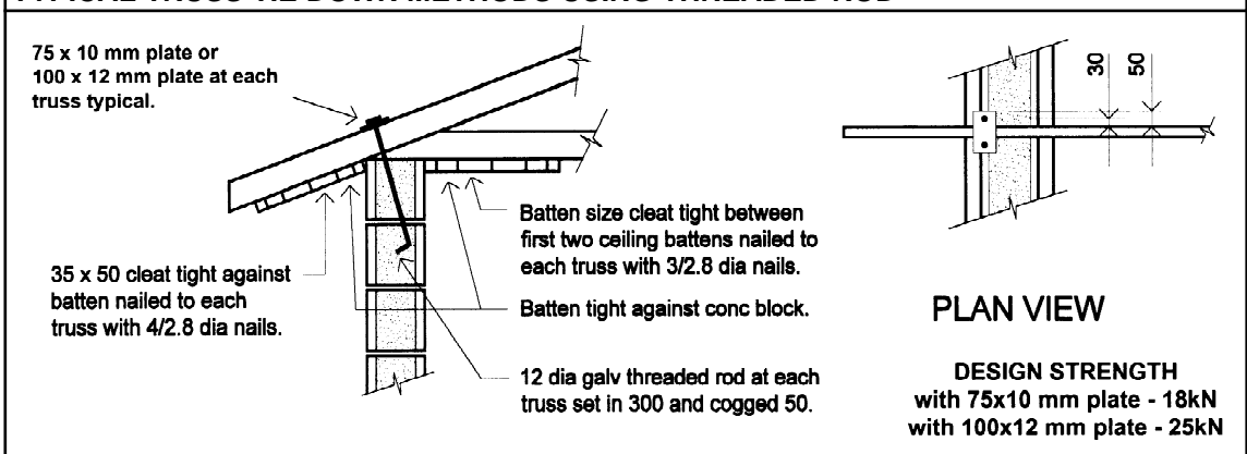
Figure 3.3.2.7(a) TYPICAL TRUSS TIE DOWN METHODS USING THREADED ROD
