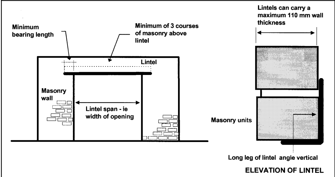
Figure 3.3.3.5 LINTELS SUPPORTING ROOFS AND MASONRY WALLS
