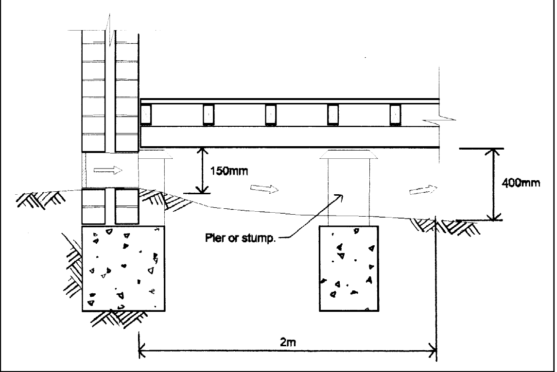
Diagram b. Sub-Floor Clearance Requirements
