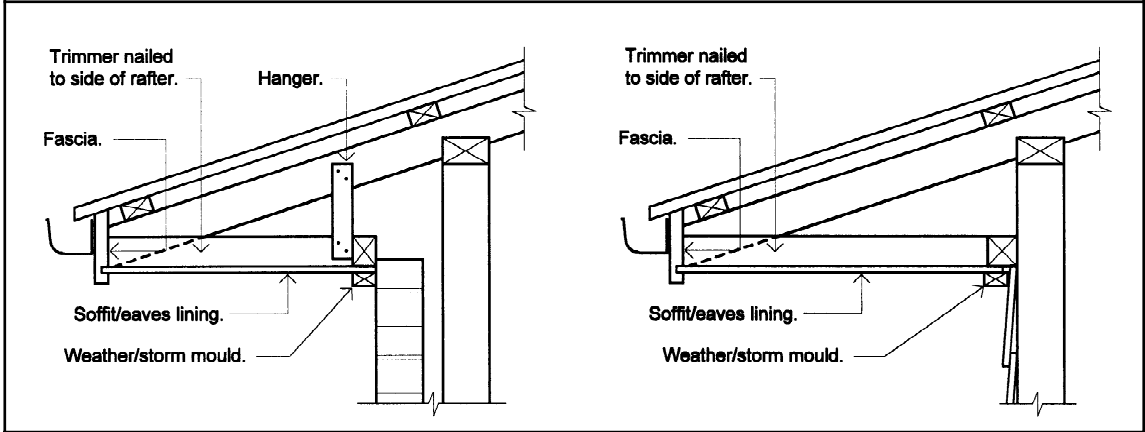
Figure 3.5.3.3 EAVES TRIMMER DETAIL
