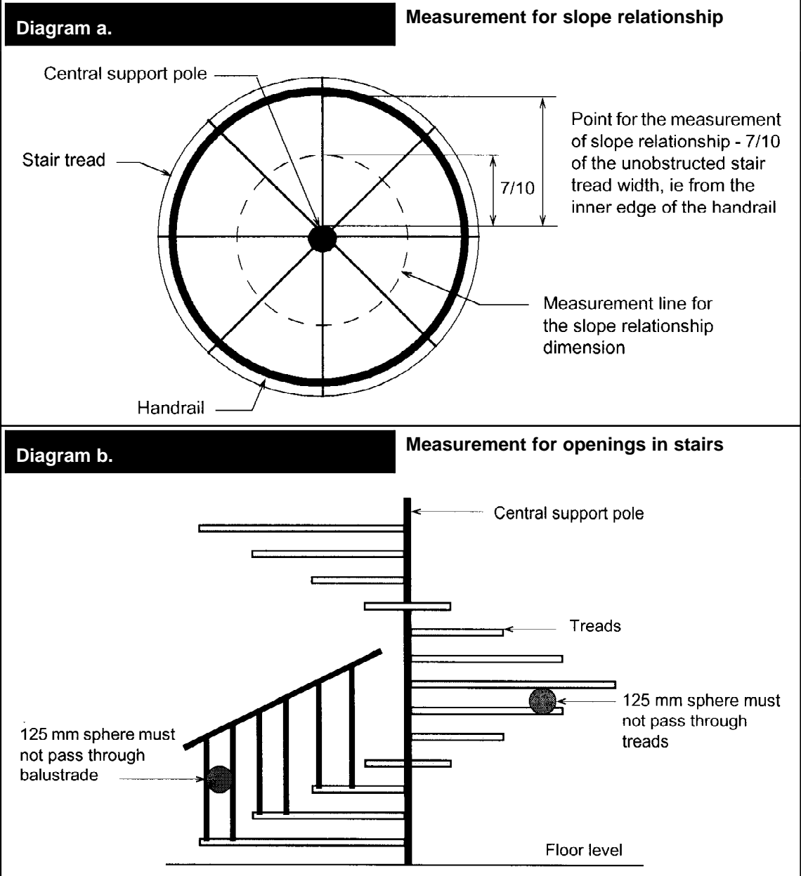
Figure 3.9.1.4 SPIRAL STAIRS
