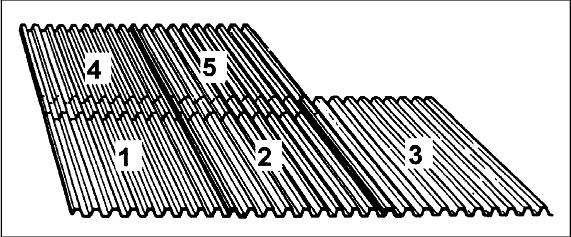
Figure 3.5.1.4 SHEET LAYING SEQUENCE
