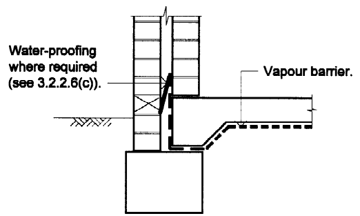
(c) Masonry alternative.
