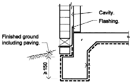
(b) Deep edge rebate alternative.
