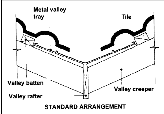
b. Dry valley
