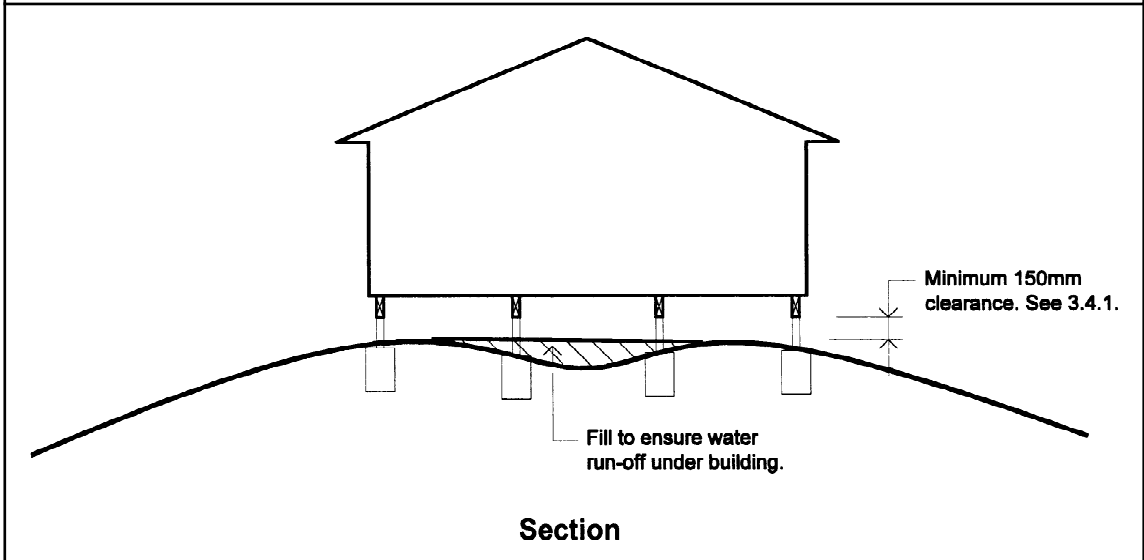
Figure 3.1.2.3 GRADING OF GROUND UNDER SUSPENDED FLOORS
