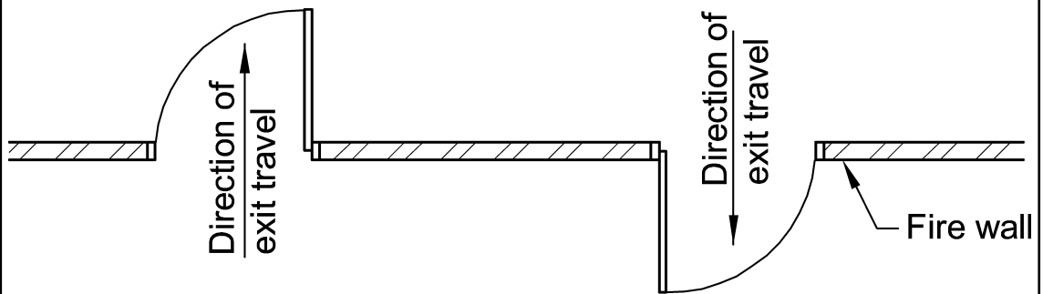
(a) Travel in both directions
