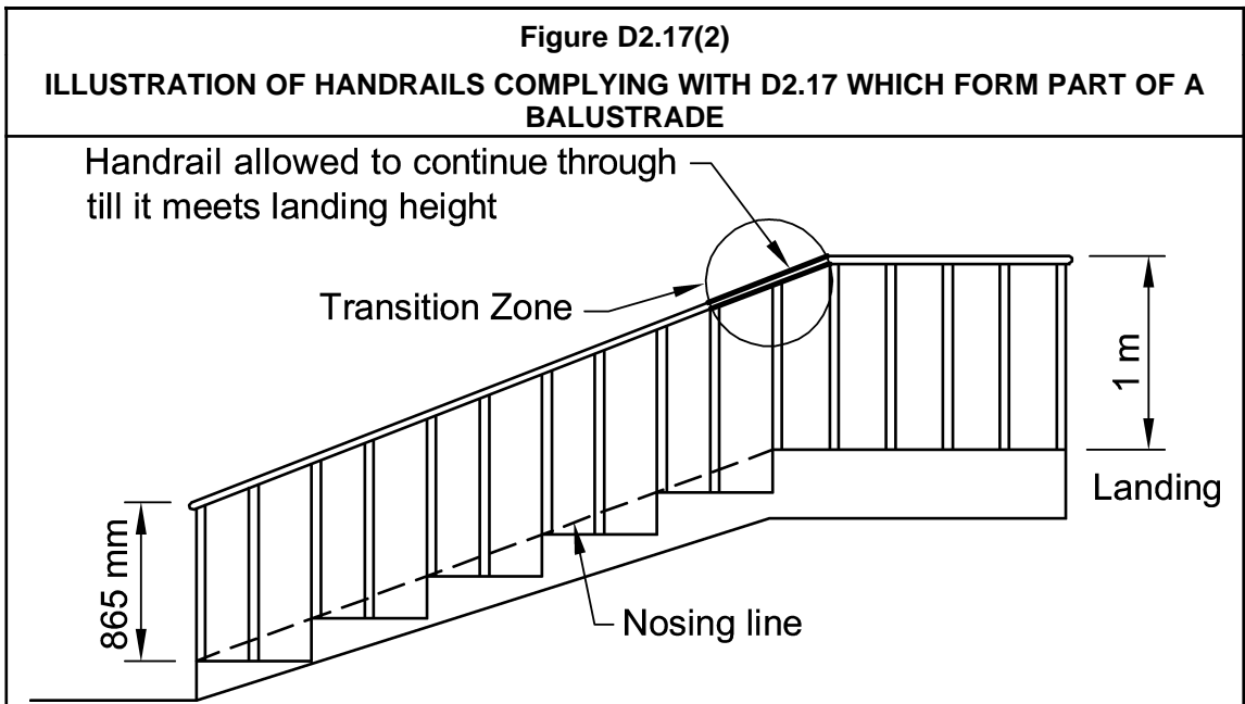
Figure D2.17(2) illustrates the use of handrails complying with D2.17 .
