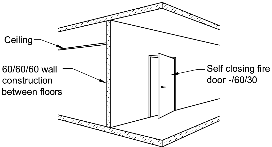
(a) Passive system
