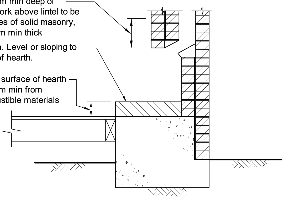
(b) Fireplace construction
