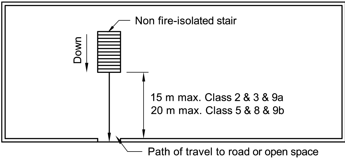
(a) Single point of egress
