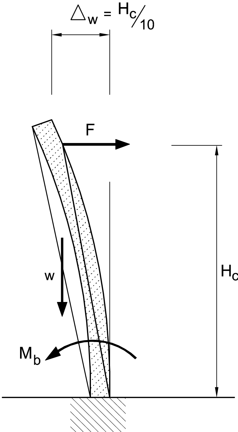
Figure C1.11(4) FORCES TO PULL PANEL INWARDS
