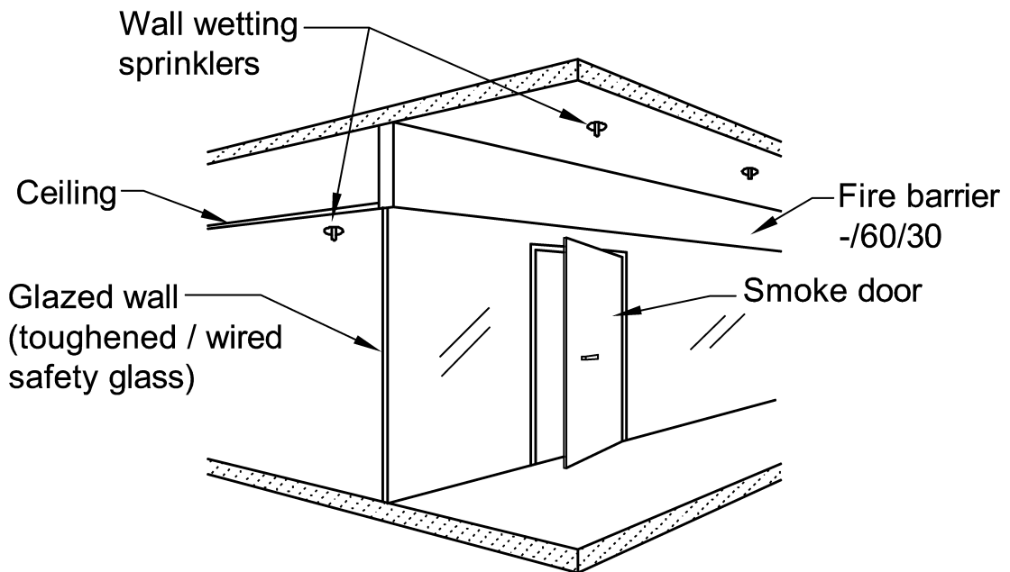
(b) Passive and active system
