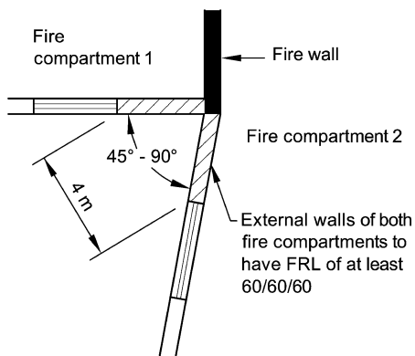
(c) External walls between 45° - 90°
