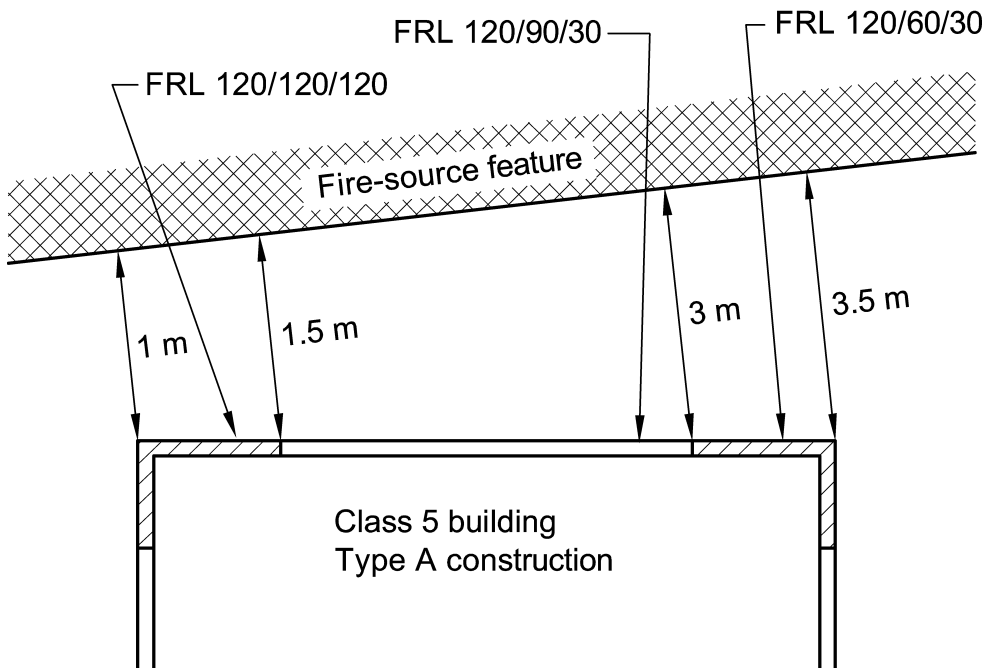
(b) Varying FRLs
