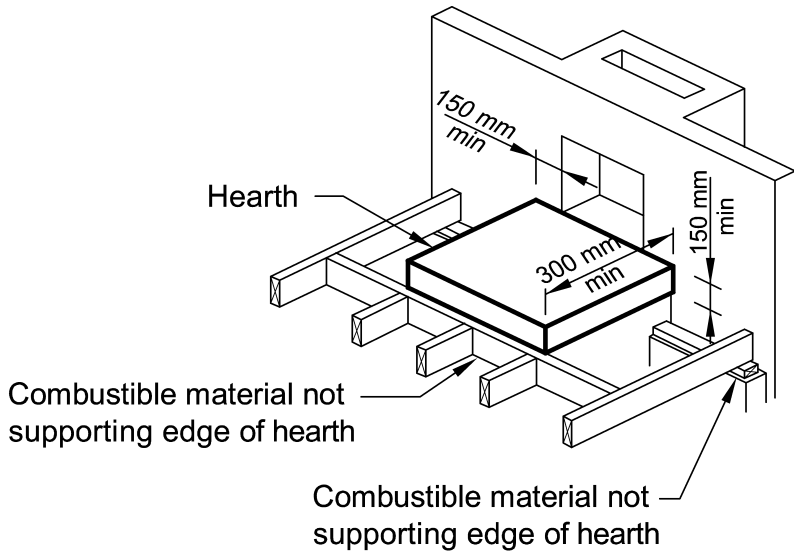
(a) Hearth construction
