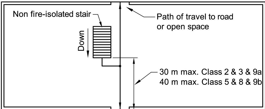
(b) Alternative points of egress
