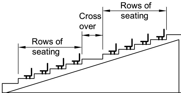
Figure C1.7 SINGLE TIERED AND TWO TIERED SEATING IN AN OPEN SPECTATOR STAND
