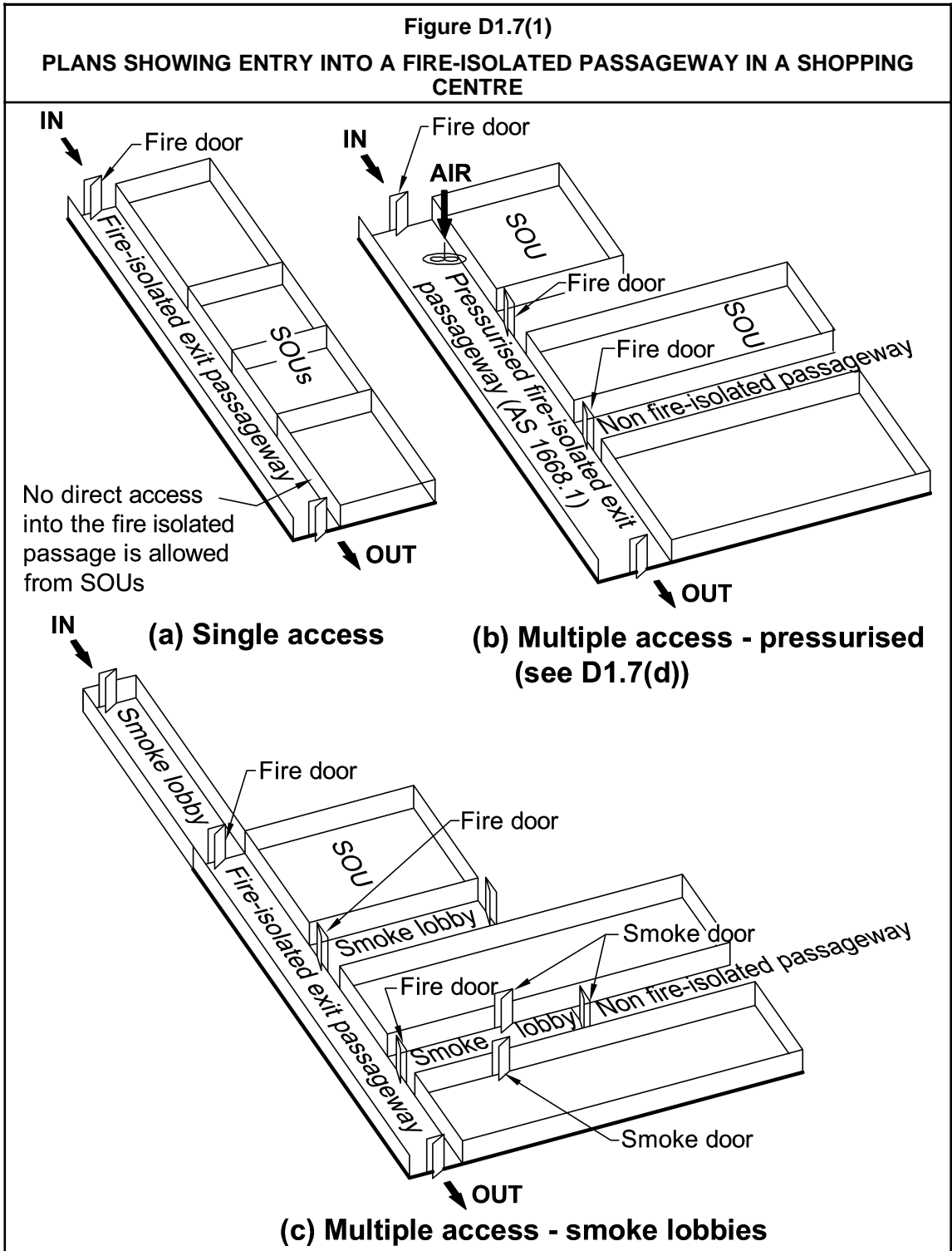
Figures D1.7(2) and (3) illustrate some of the options available by the use of D1.7.
