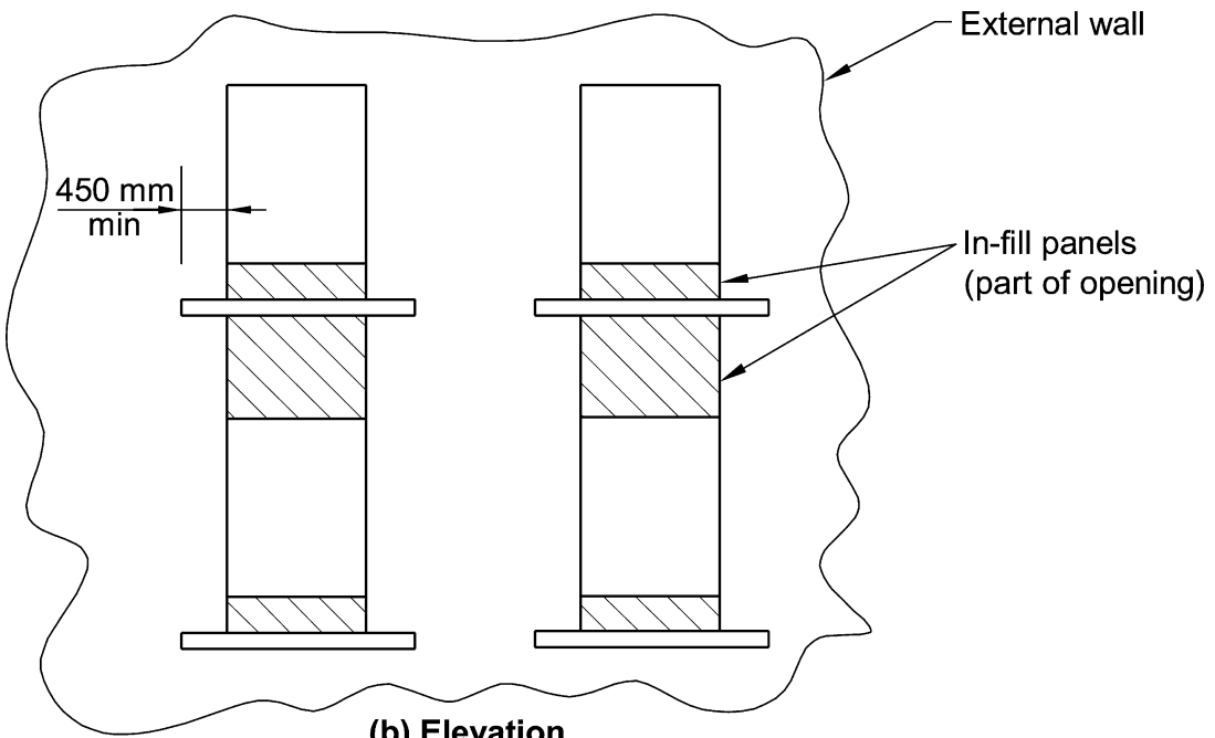
(b) Elevation
