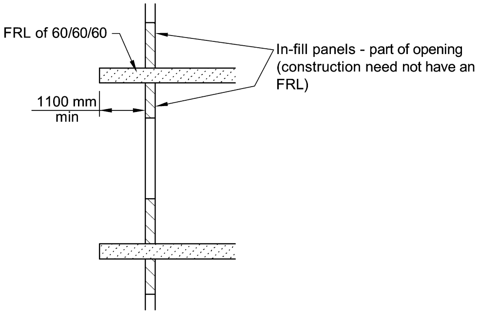
(a) Section
