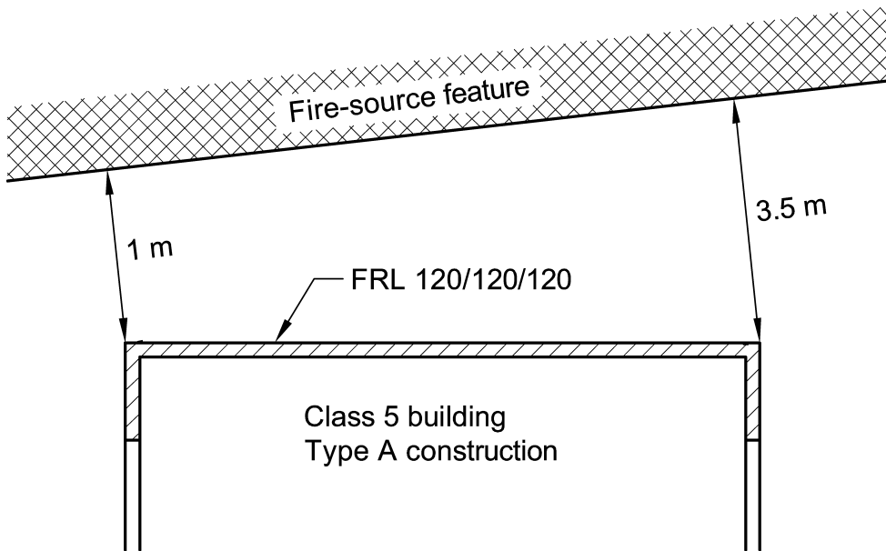
(a) Single FRL
