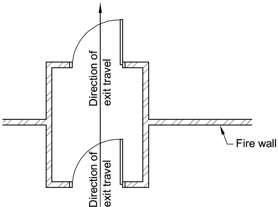
(a) Travel in both directions
