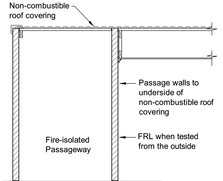
(a) Wall extending to roof covering
