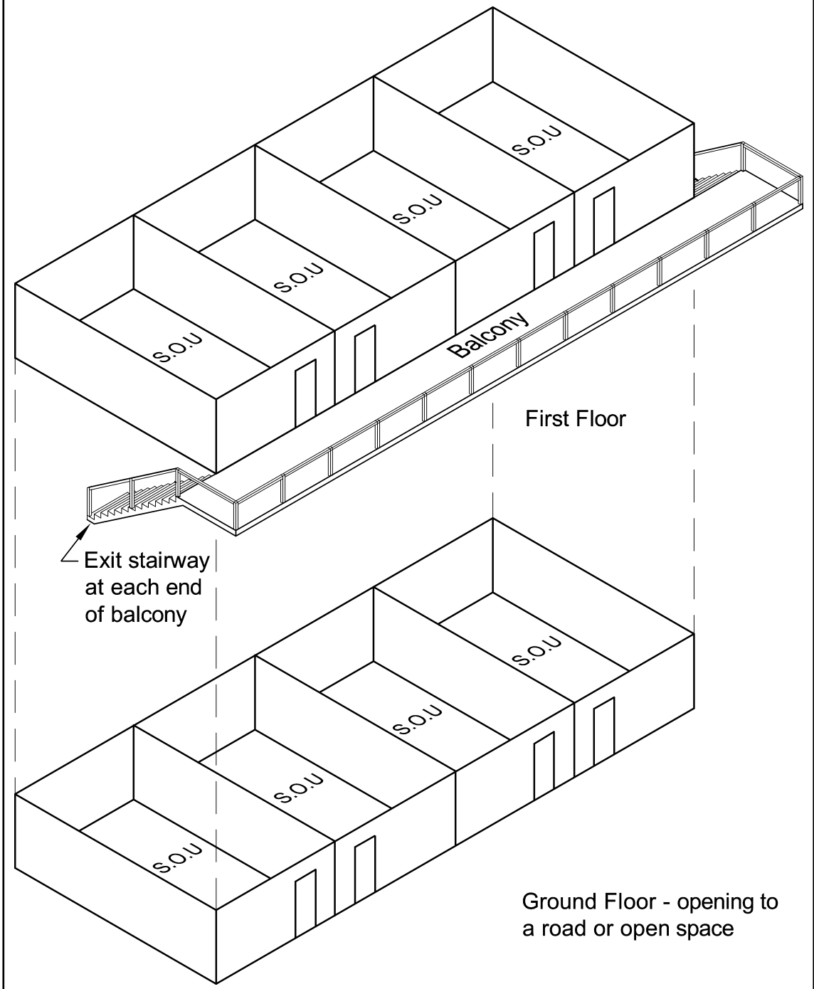
Figure C1.5 EXAMPLE OF THE CONCESSION ALLOWED BY C1.5
