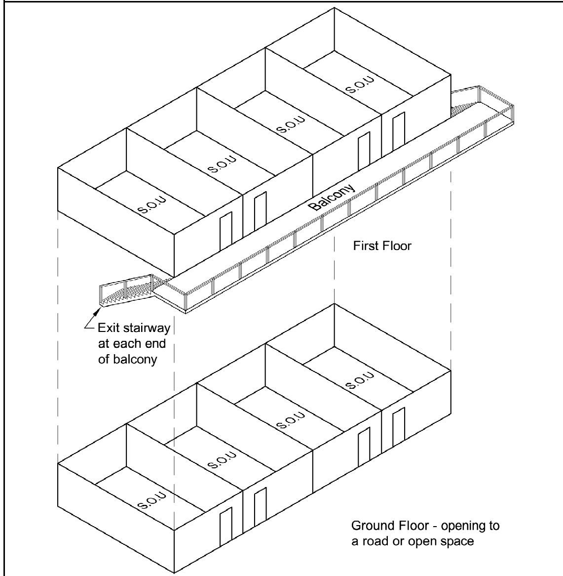
Figure C1.5 EXAMPLE OF THE CONCESSION ALLOWED BY C1.5
