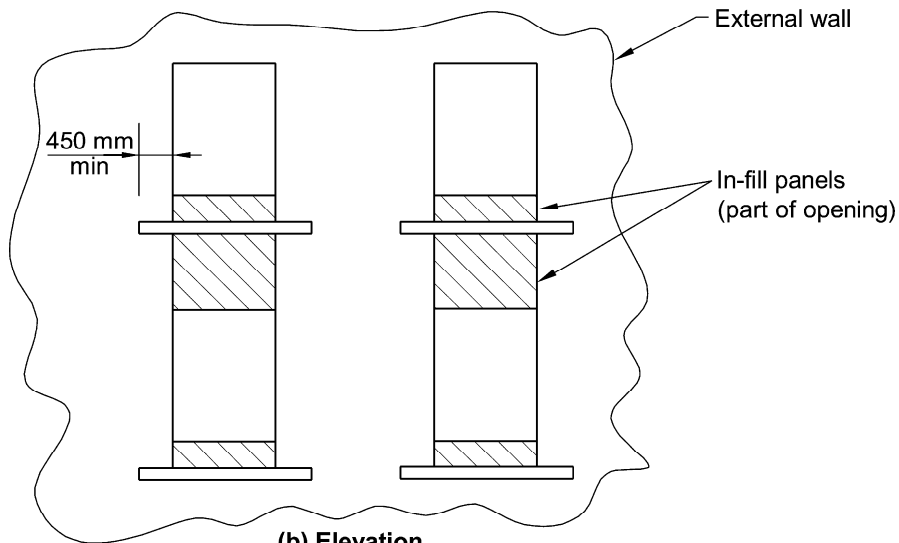
(b) Elevation
