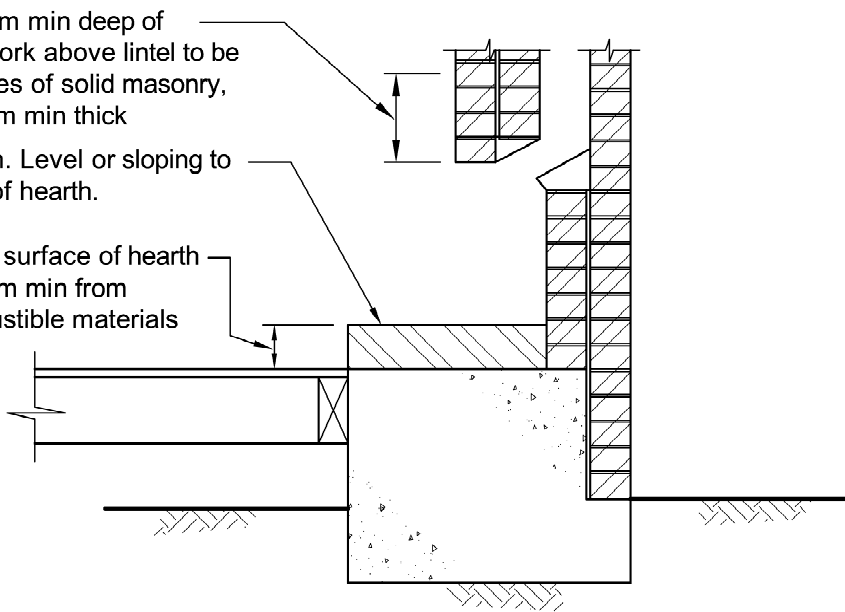
(b) Fireplace construction
