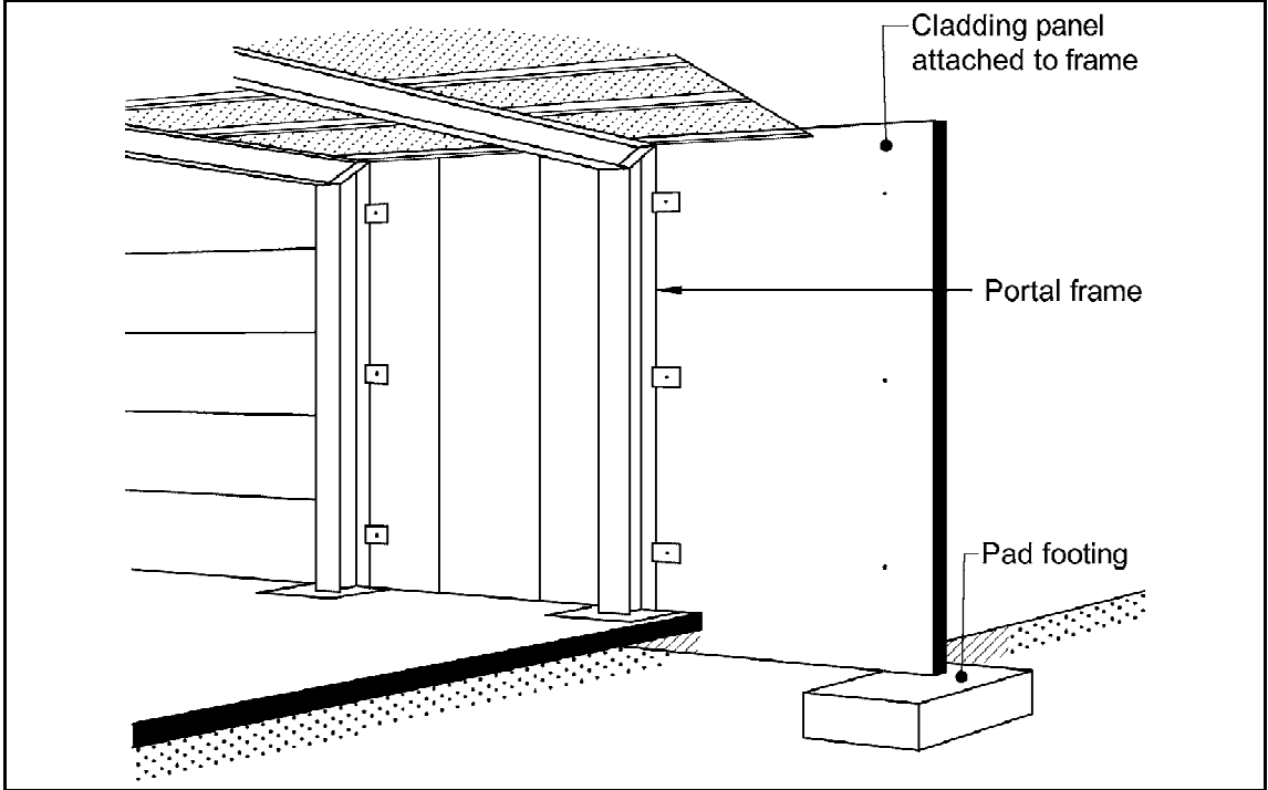
Figure Spec C1.11(1) TYPICAL NON-LOADBEARING PANELS REQUIRED TO COMPLY WITH SPECIFICATION C1.11 (PANELS MAY BE FULL BAY, MULTIPLE VERTICALLY OR HORIZONTALLY SPANNING)
