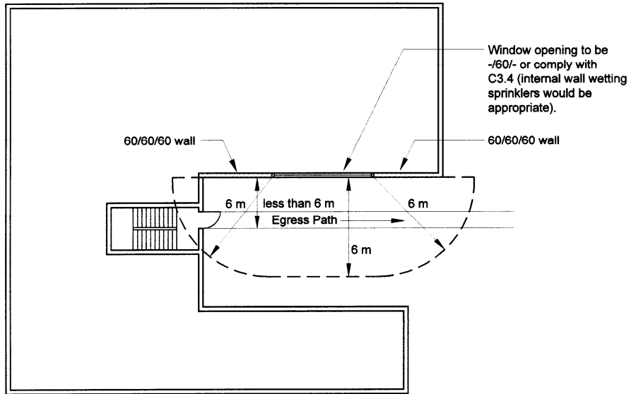
Case 3 - Protection of wall and openings.
