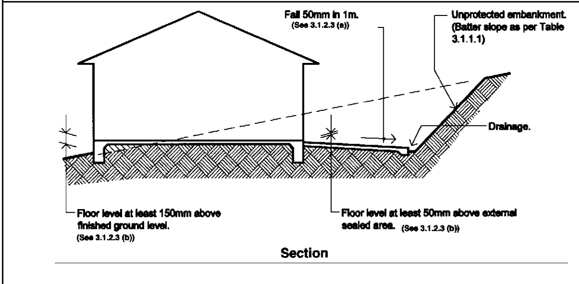
Figure 3.1.2.2 SITE SURFACE DRAINAGE
