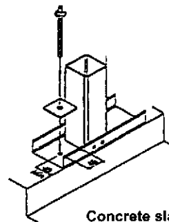
Concrete slab - Sheet roof Chemical anchor with washer
