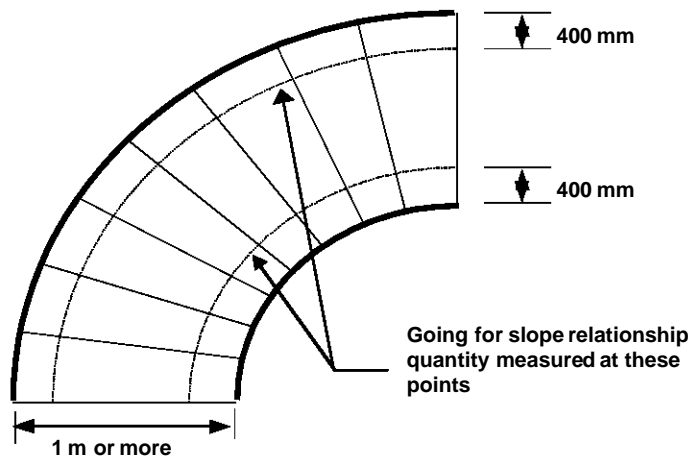
Diagram c. Tapered treads - 1 m or more in width
