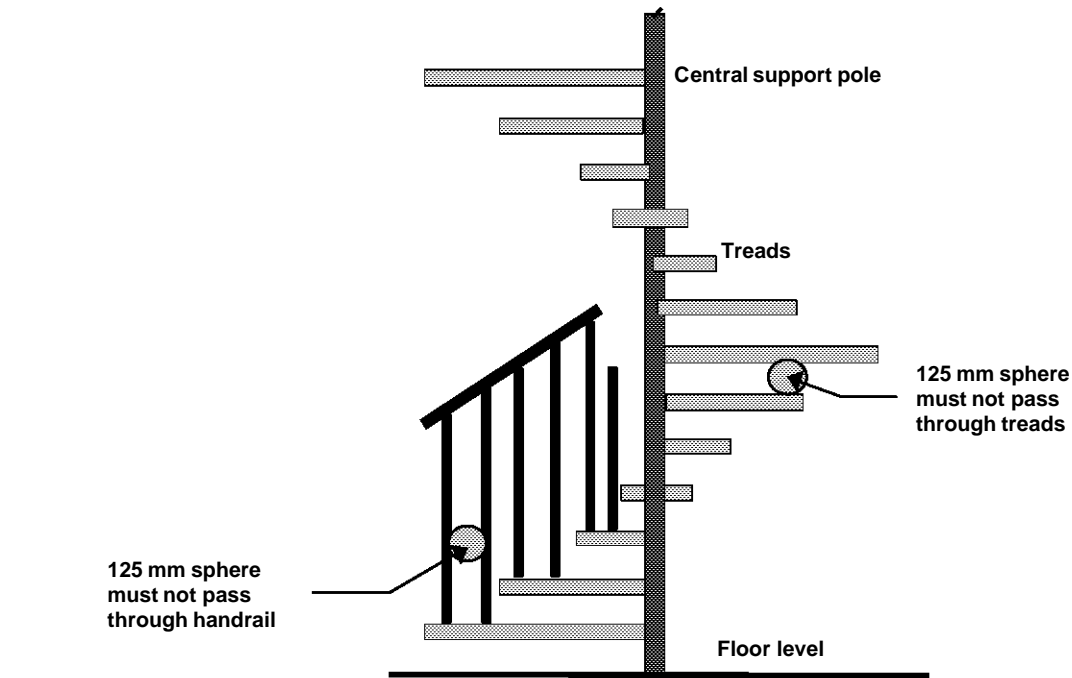
Diagram b. Measurement for openings in stairs
