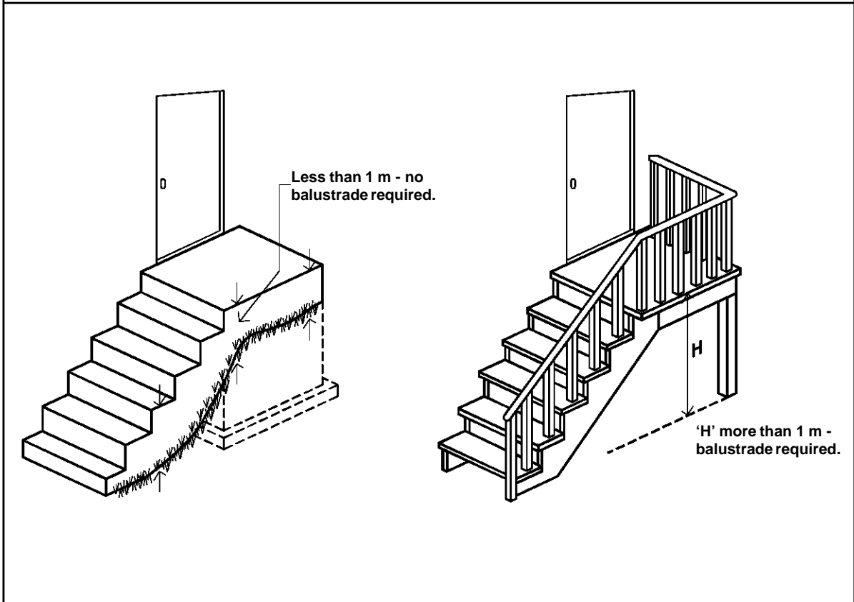
Figure 3.9.2.3 BALUSTRADES - WHEN REQUIRED
