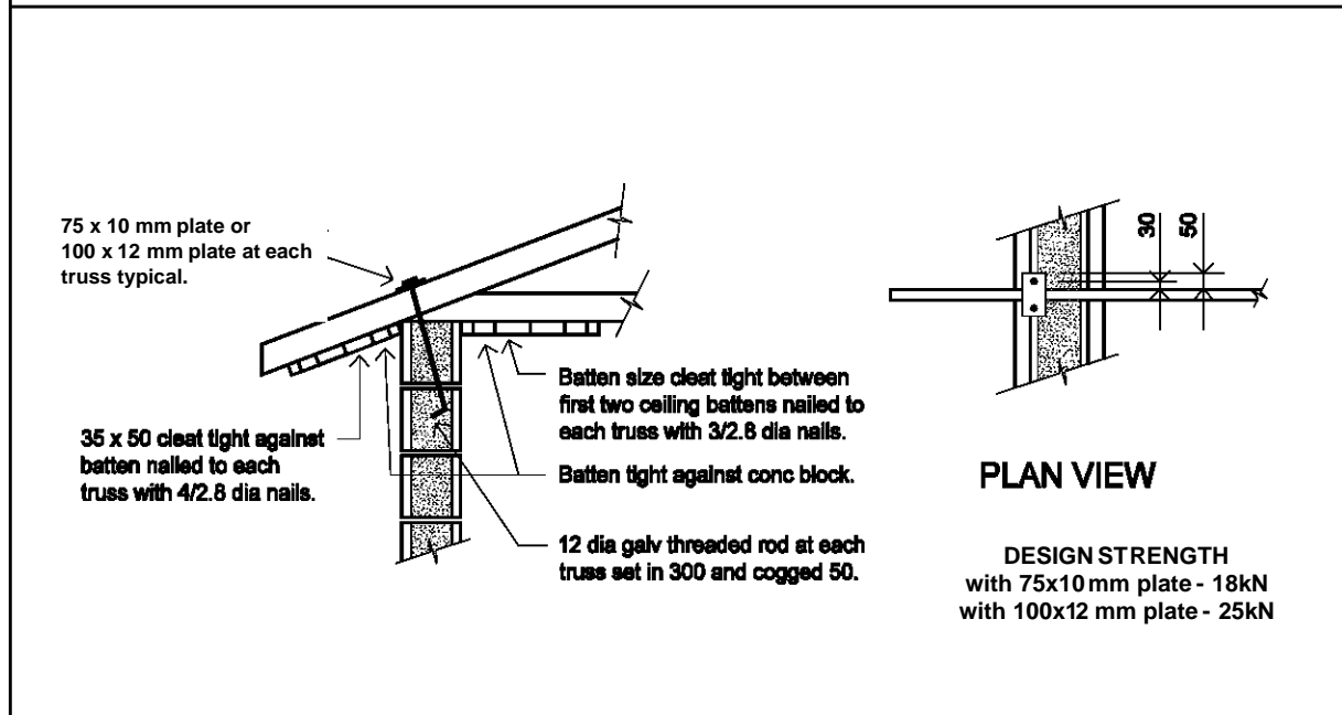
Figure 3.3.2.7(a) TYPICAL TRUSS TIE DOWN METHODS USING THREADED ROD
