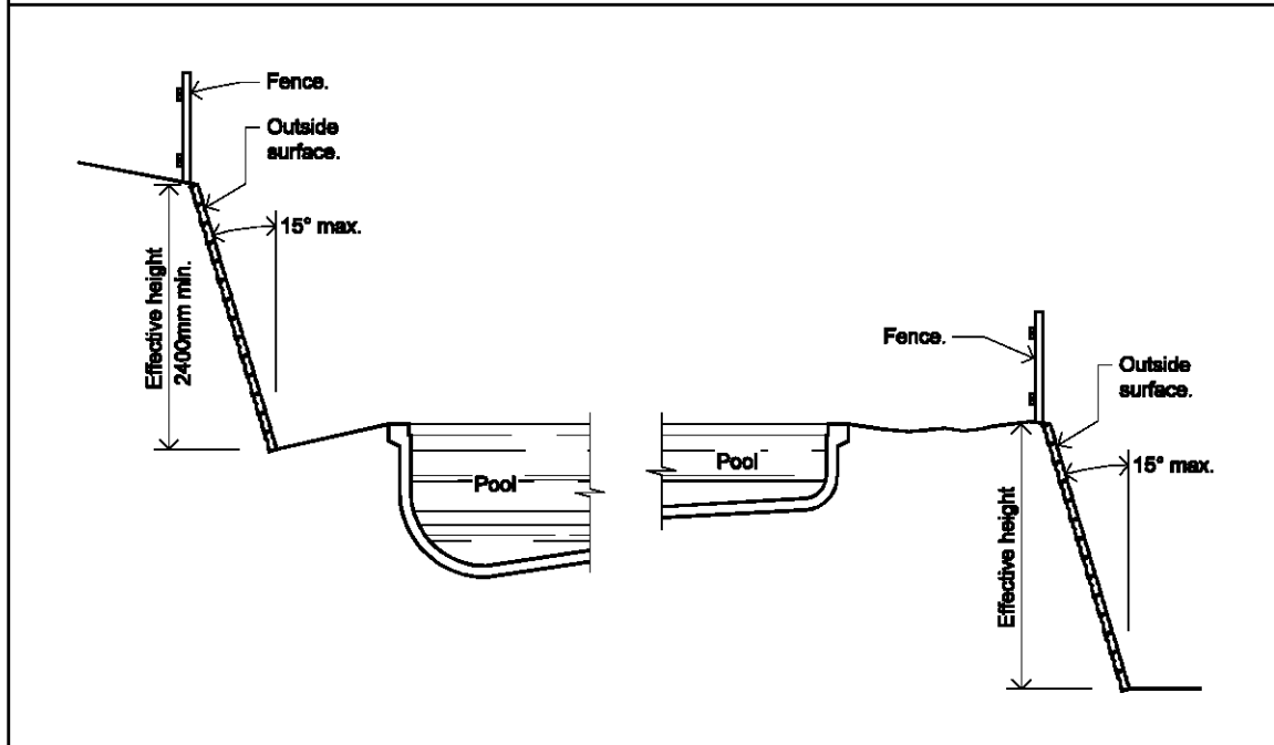
Figure 3.9.3.5 RETAINING WALLS AND OTHER SUCH BARRIERS
