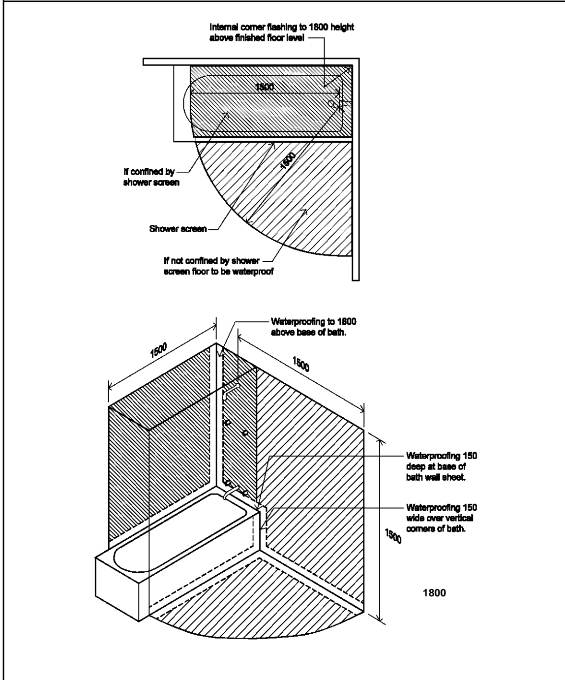
Figure 3.8.1.2 SHOWERS ABOVE BATHS - AREA TO BE PROTECTED
