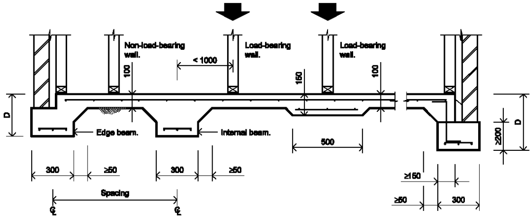
REINFORCEMENT FOR STIFFENED RAFT FOR CLASS A, S AND M SITES
