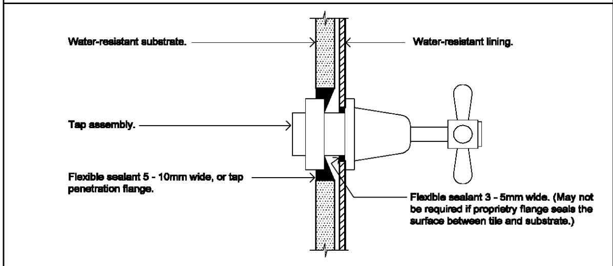
Figure 3.8.1.6 TYPICAL INSTALLATION OF TAP FLANGE
