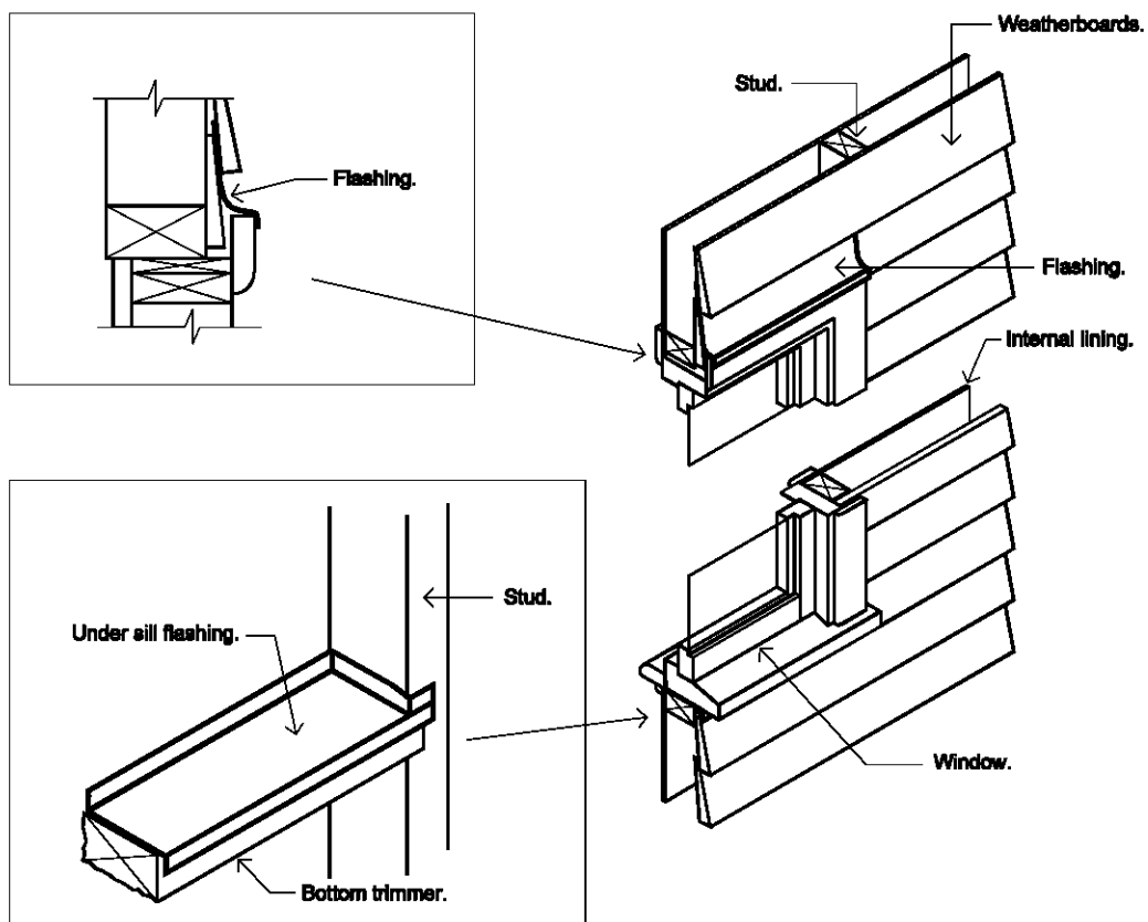
Figure 3.5.3.4 TYPICAL WINDOW FLASHING DETAIL
