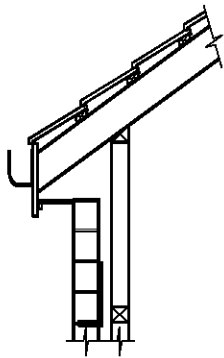
CONSTRUCTION TYPE A
