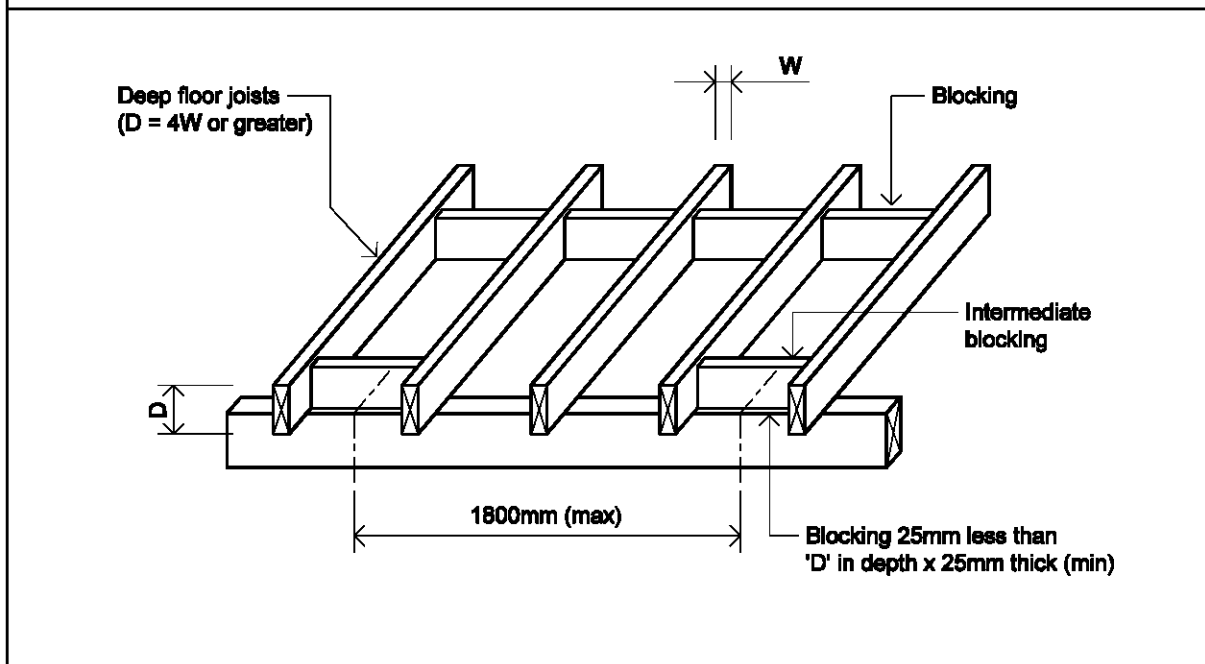
Figure 3.4.3.4 BLOCKING FOR DEEP JOISTS
