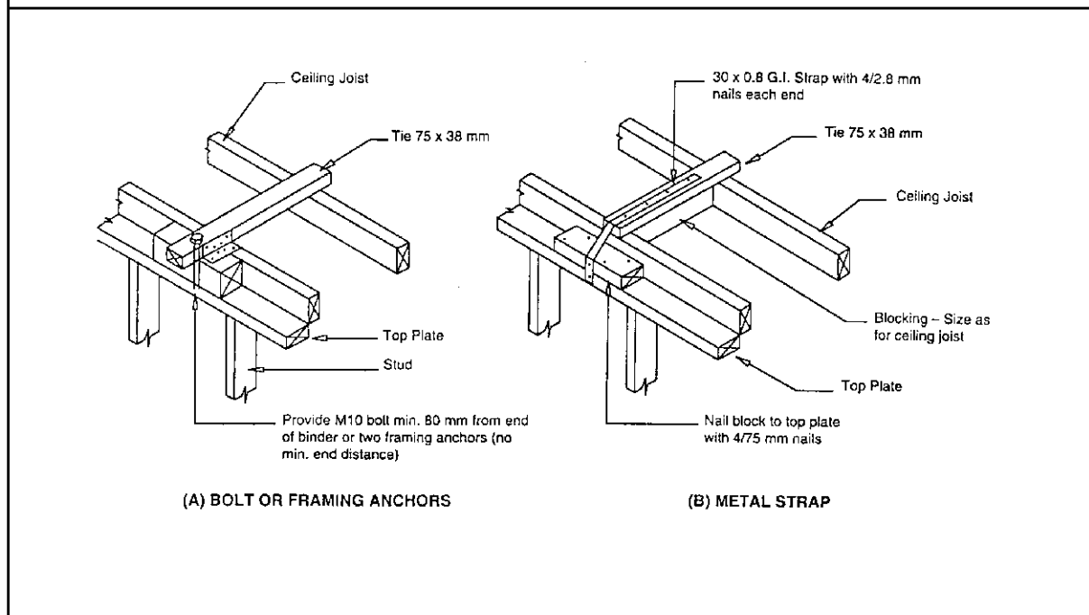
Figure 3.4.3.9 BINDERS TO CONNECT WALLS TO CEILING FRAME
