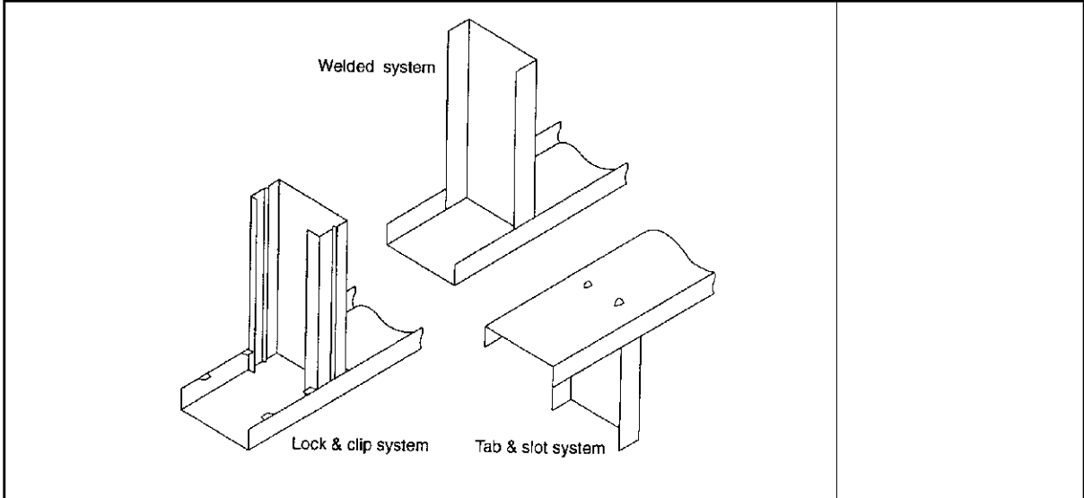
Figure 3.4.2.2 TYPICAL WALL FRAMING AND SECTION MEMBERS
