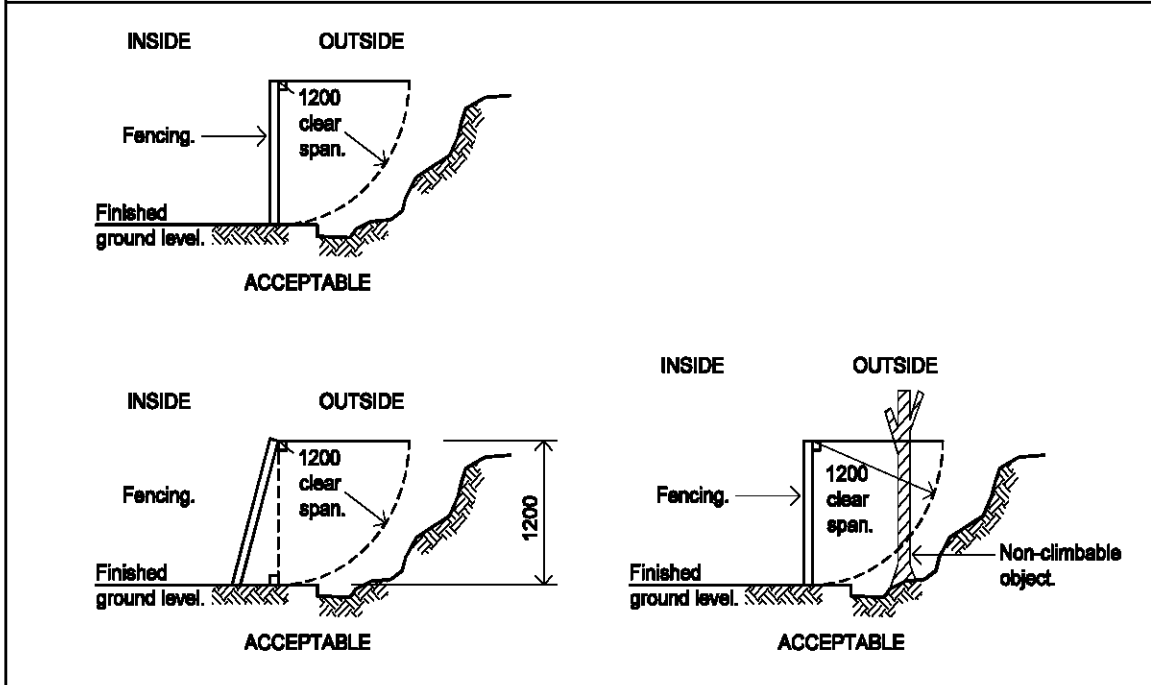
Figure 3.9.3.4 EFFECTIVE FENCING HEIGHT
