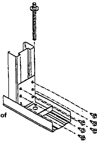
Diagram b. For Areas With A Design Wind Speed Of More Than W41
