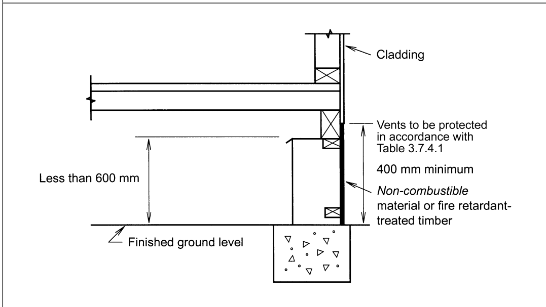
Figure 3.7.4.1 PROTECTION OF SUB-FLOOR SPACES WITH LESS THAN 600 MM CLEARANCE
