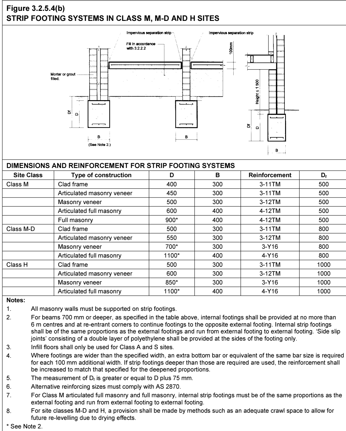
Figure 3.2.5.4(b) Amdt No. 6
