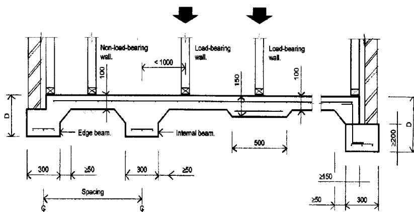
Figure 3.2.5.3(b) FOOTING SLAB AND STIFFENED RAFT SLAB DETAILS FOR CLASS M, M-D, H AND H-D SITES
