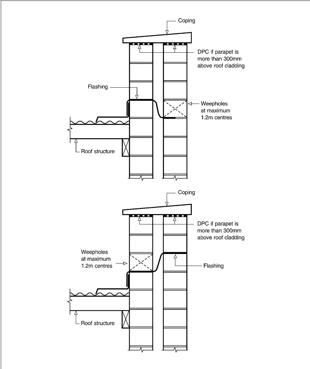
Figure 3.3.4.2 INSTALLATION OF DPCs AND FLASHINGS FOR PARAPET WALLS
