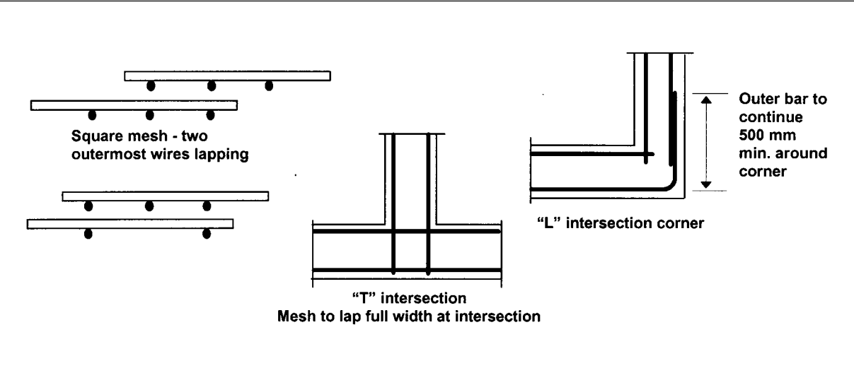
Figure 3.2.3.1 LAPS IN REINFORCEMENT
