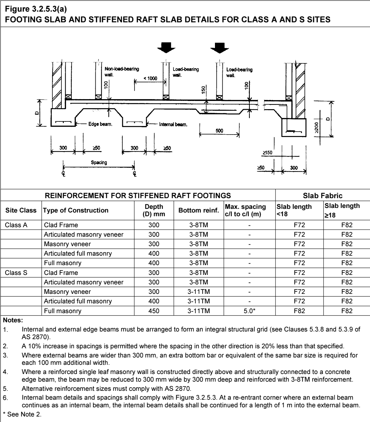
Figure 3.2.5.3(a) Amdt No. 6
