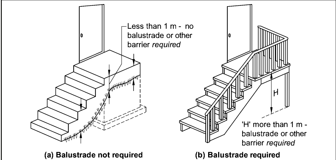
Figure 3.9.2.3 BALUSTRADES OR OTHER BARRIERS — WHEN REQUIRED
