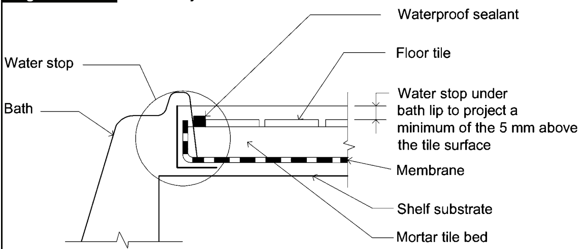
Diagram c Bath/shelf junction
