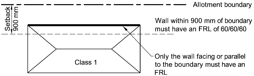
Diagram b. Part walls protection
