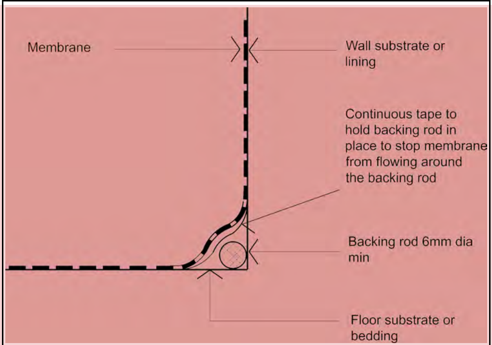
TYPICAL BOND BREAKER DETAIL FOR CLASS I MEMBRANES
