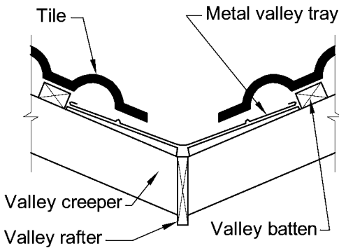
Standard arrangement
