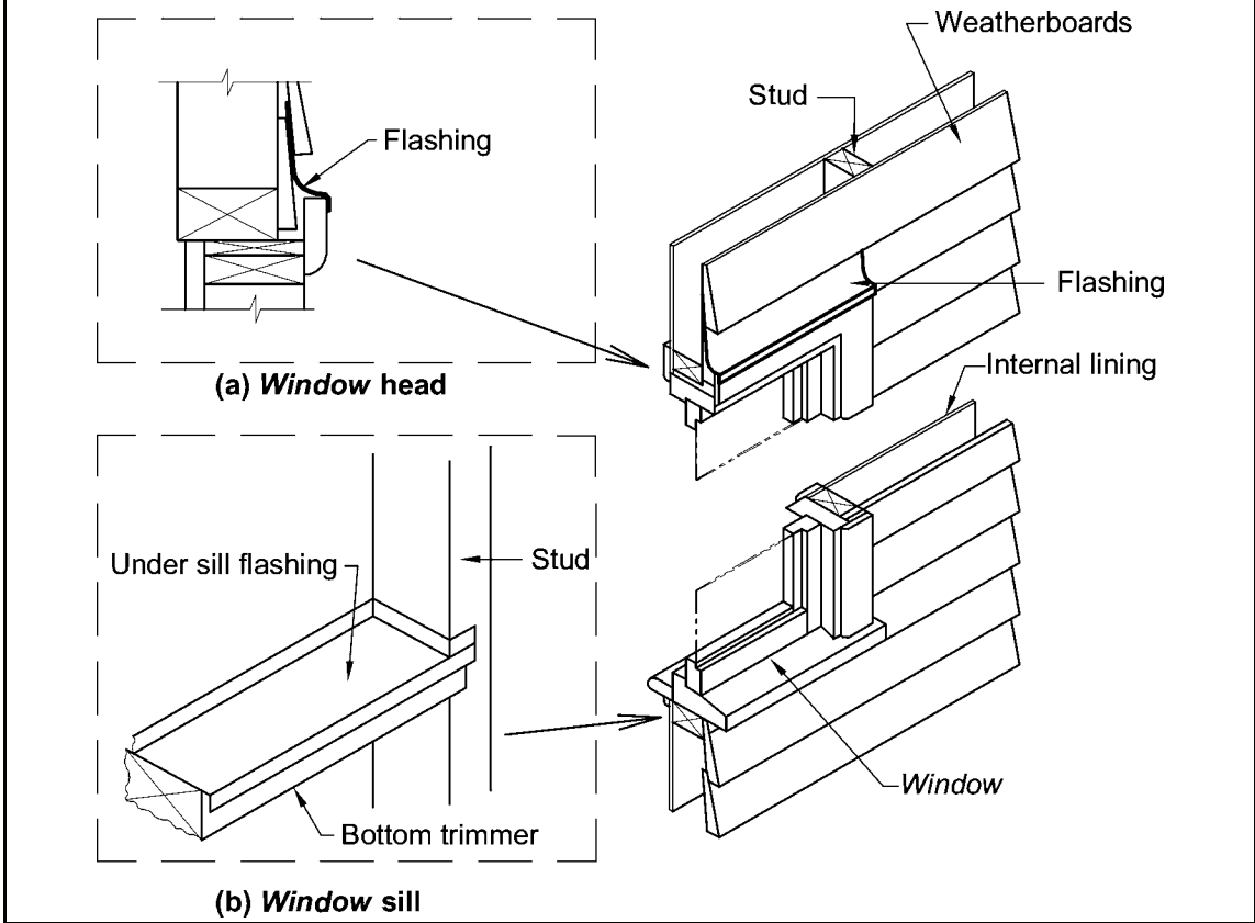
Figure 3.5.3.4 TYPICAL WINDOW FLASHING DETAIL
