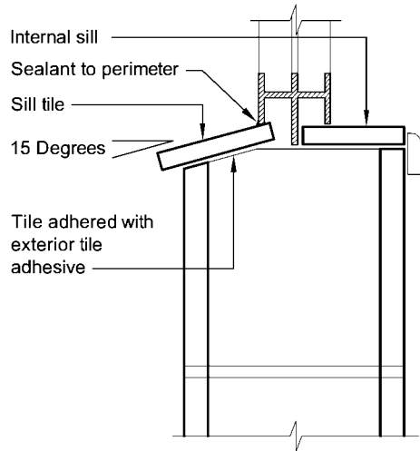
(c) Sill fixing - 1
