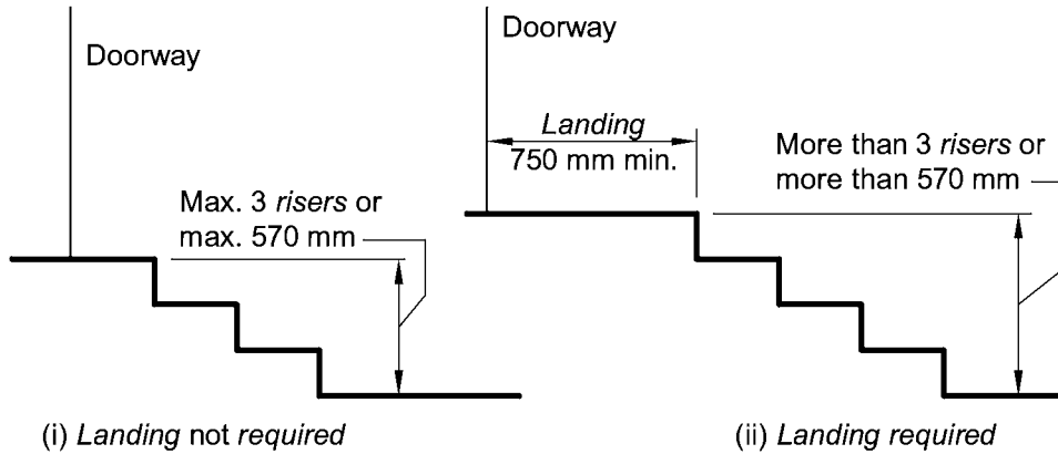
Diagram b. Threshold landing
