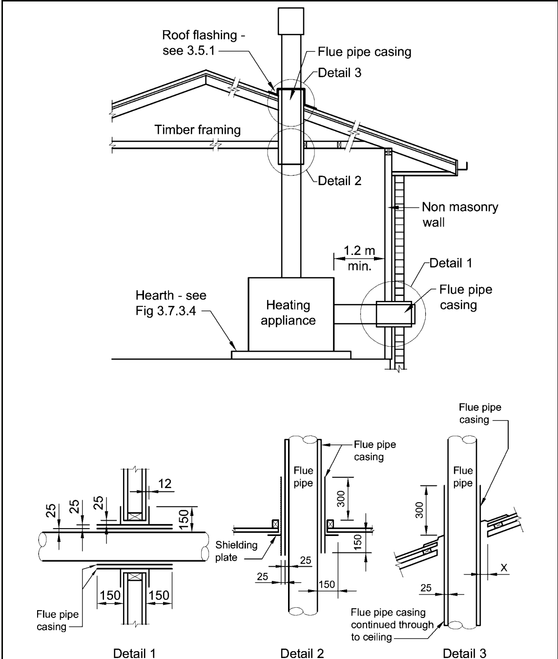
Figure 3.7.3.5 ACCEPTABLE FLUE INSTALLATION DETAILS
