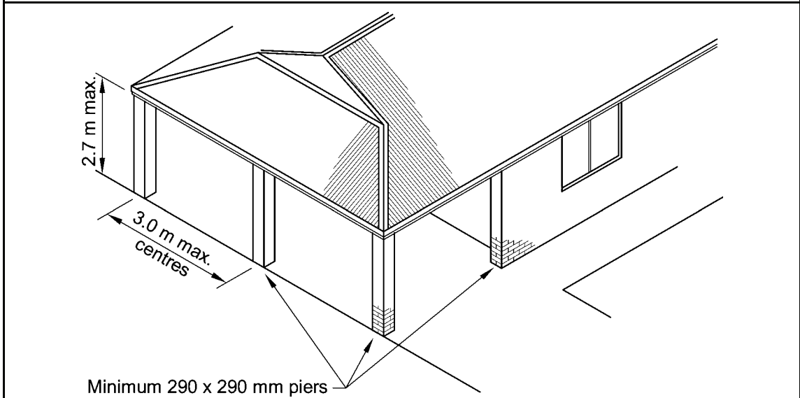
Figure 3.3.1.5 ISOLATED PIERS UNDER MAIN ROOF
