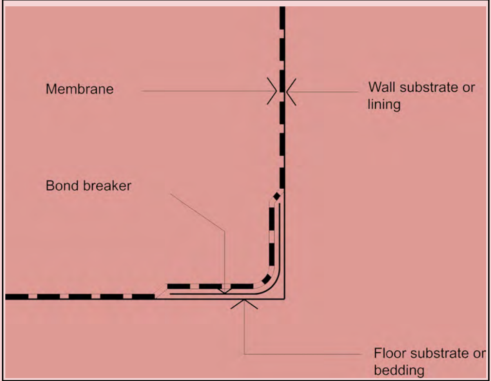
TYPICAL BOND BREAKER DETAIL FOR CLASS II MEMBRANES
