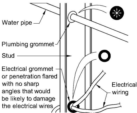
(c) Penetration protection
