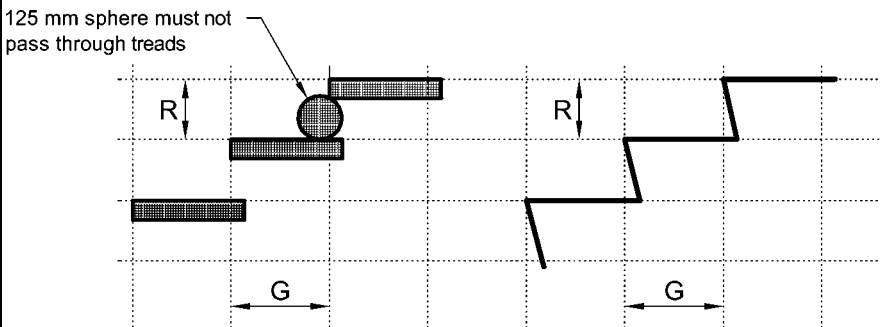
Figure 3.9.1.2 STAIR RISER AND GOING DIMENSIONS (mm)
