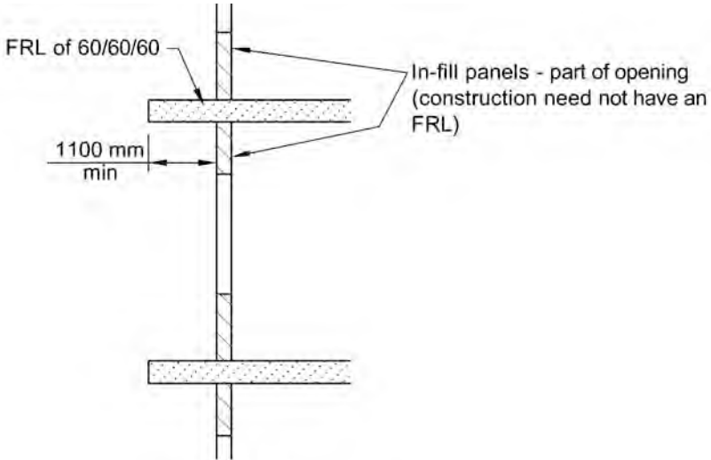
(a) Section
