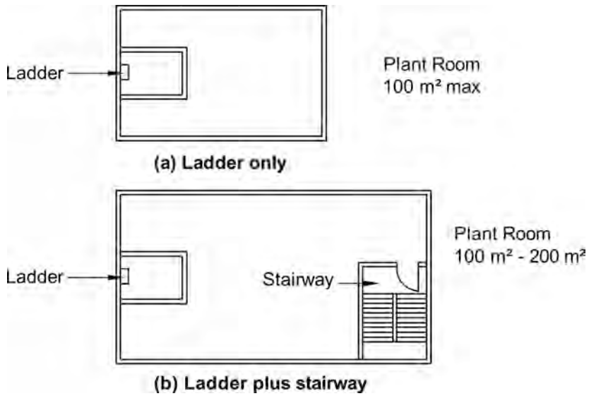
Figure D1.16 PLANS SHOWING USE OF D1.16
