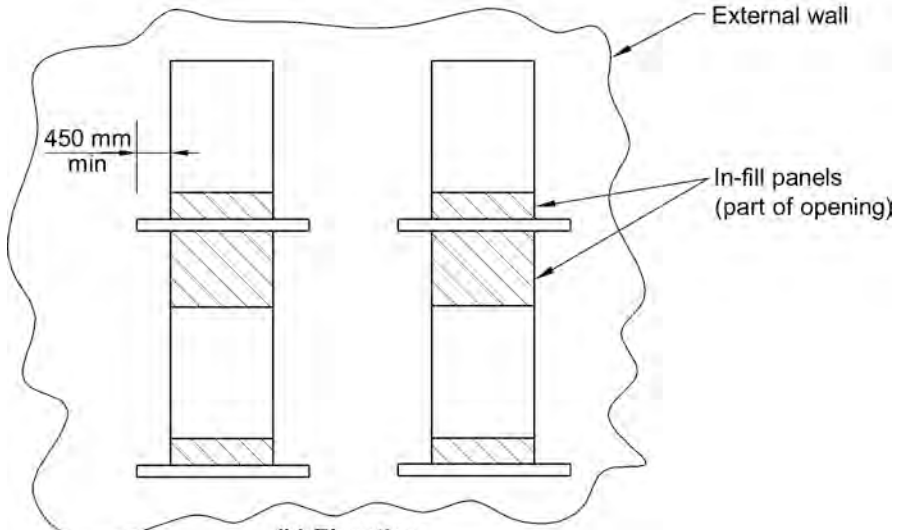
(b) Elevation
