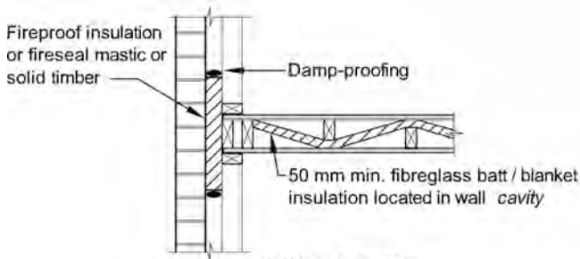
(c) Plan detail
