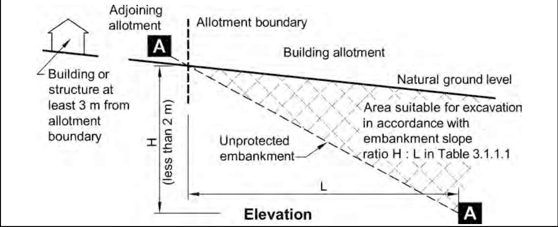
Figure 3.1.1.1 EXCAVATION AFFECTING ADJOINING PROPERTY
