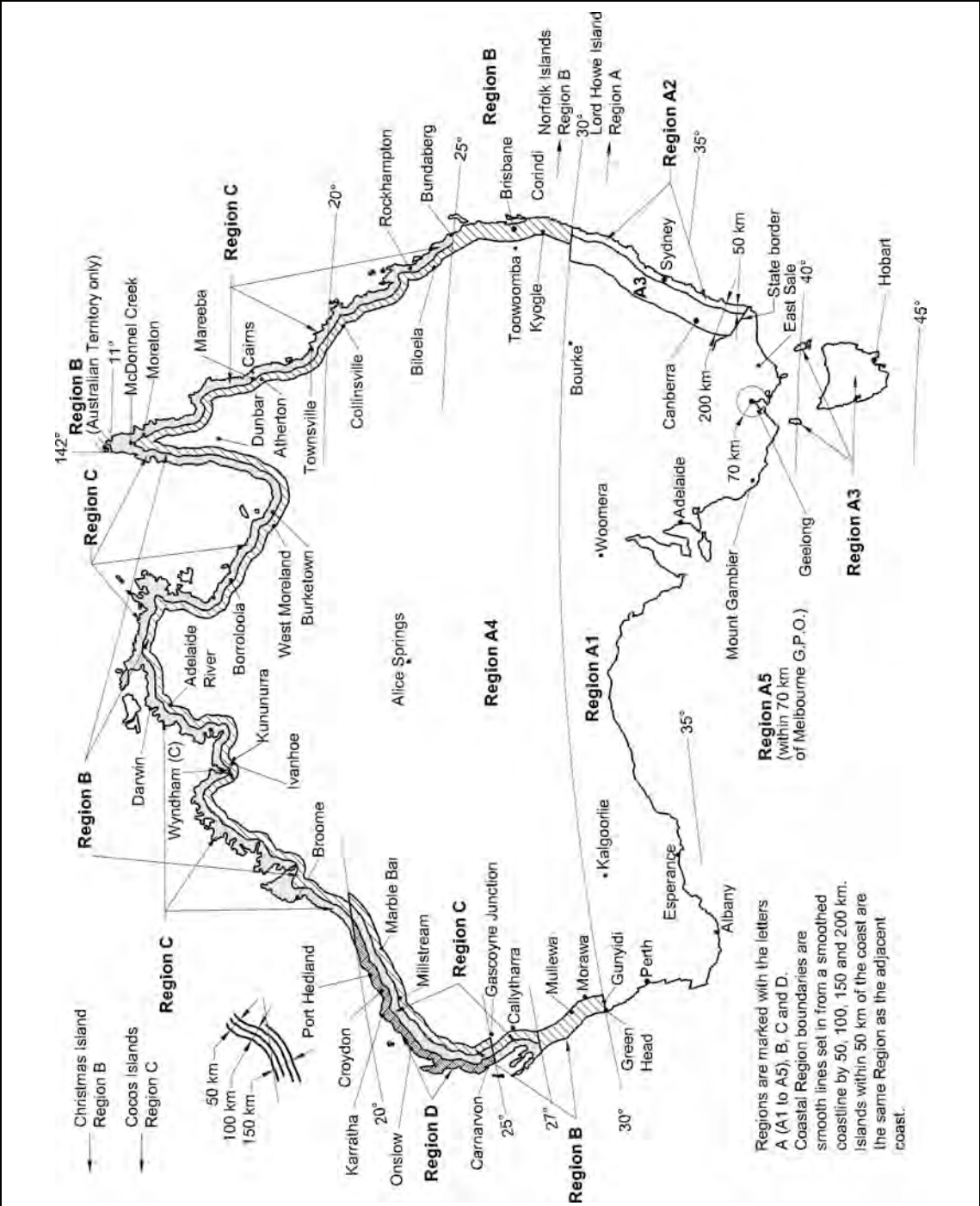
Figure 3.10.1.4 WIND REGIONS
