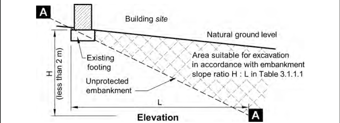
Figure 3.1.1.2 EXCAVATION ADJACENT TO EXISTING BUILDINGS
