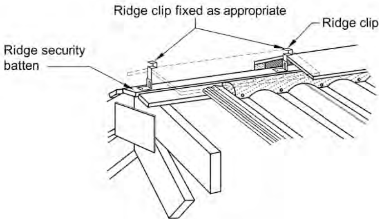
Diagram a. Mechanical fastening-ridge clip (Also see Figure 3.5.1.1 )
