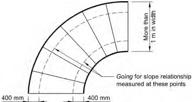
Diagram c. Tapered treads — more than 1 m in width
