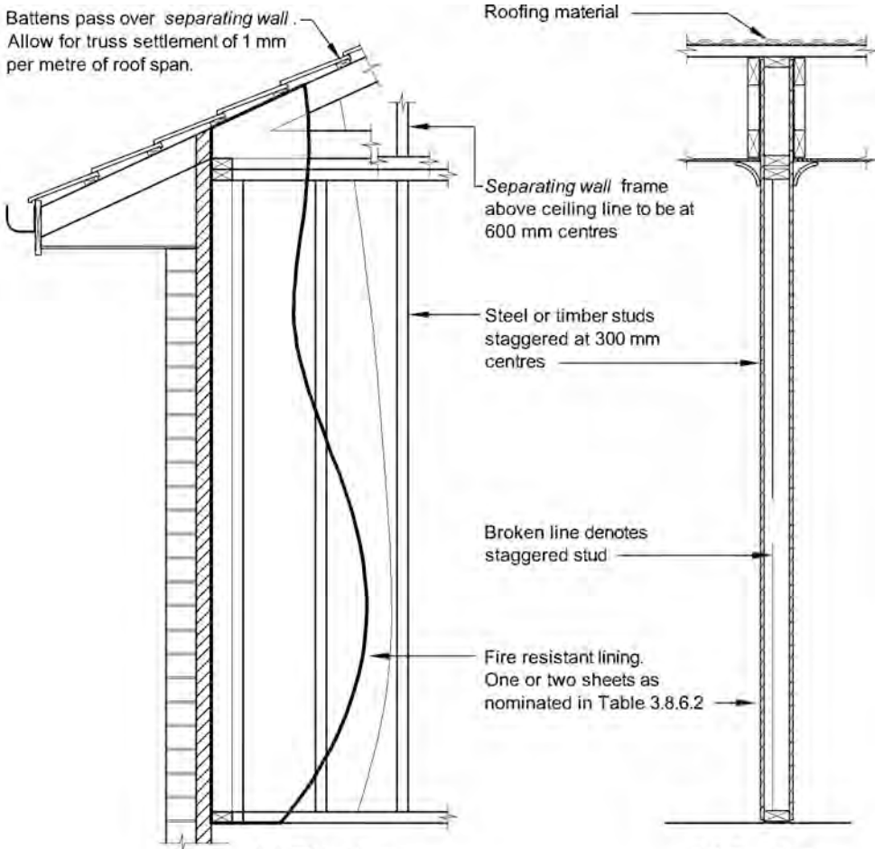
(a) Elevation
