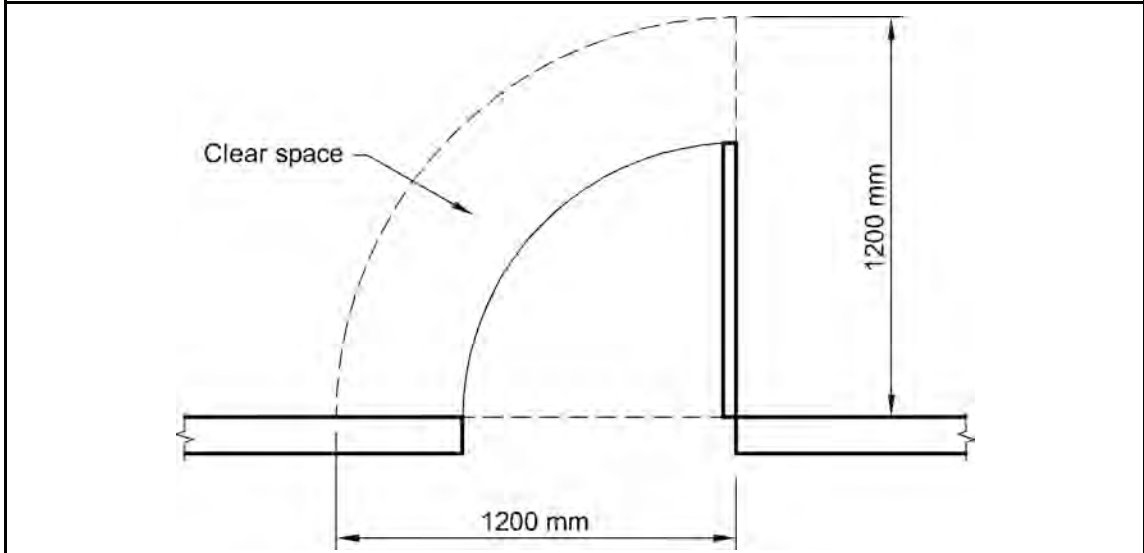
Figure 3.8.3.3 CONSTRUCTION OF SANITARY COMPARTMENTS
