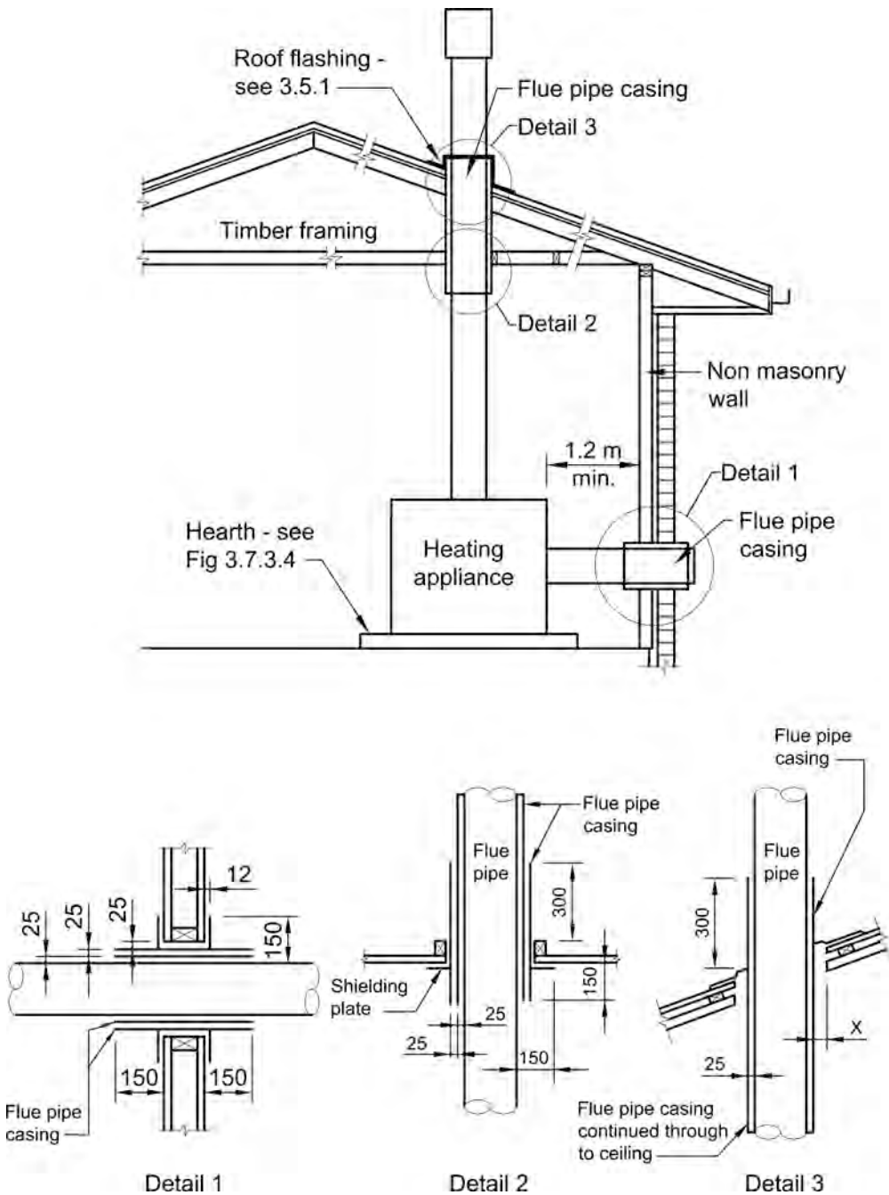
Figure 3.7.3.5 ACCEPTABLE FLUE INSTALLATION DETAILS
