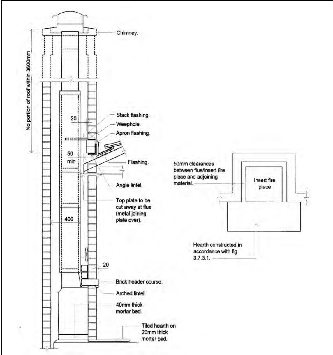
Figure 3.7.3.3 TYPICAL INSTALLATION OF FIRE PLACE FLUE INSERTS
