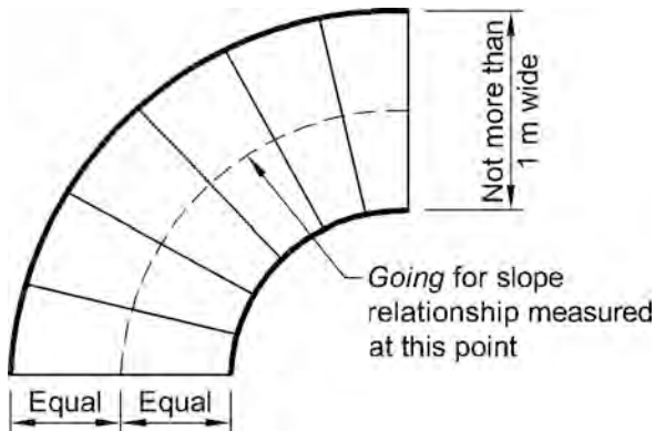
Diagram b. Tapered treads — not more than 1 m wide
