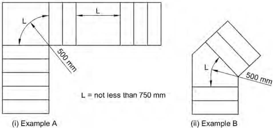
Diagram a. Stairway landing
