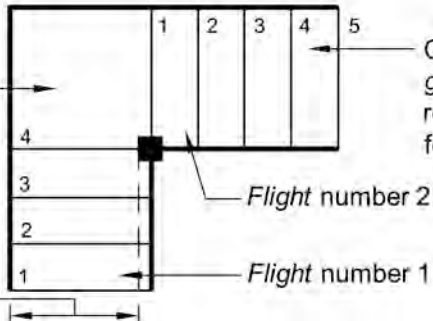
Diagram b. Tapered treads — not more than 1 m wide
