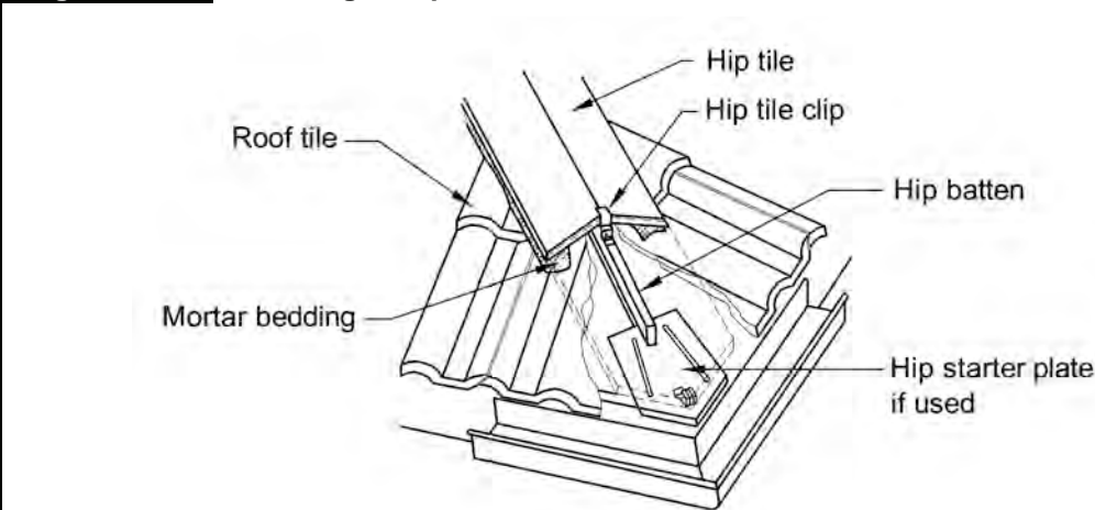
Diagram d. Fastening of hip tiles
