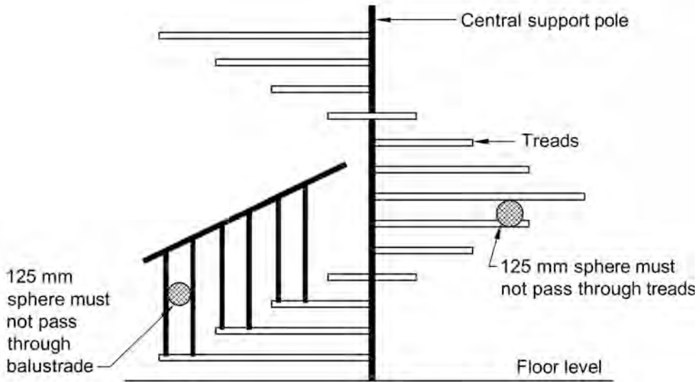
Figure 3.9.1.5 LANDINGS
