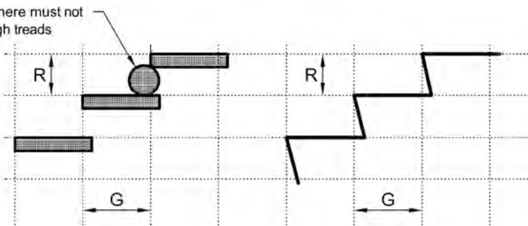
Figure 3.9.1.2 STAIR RISER AND GOING DIMENSIONS (mm)
