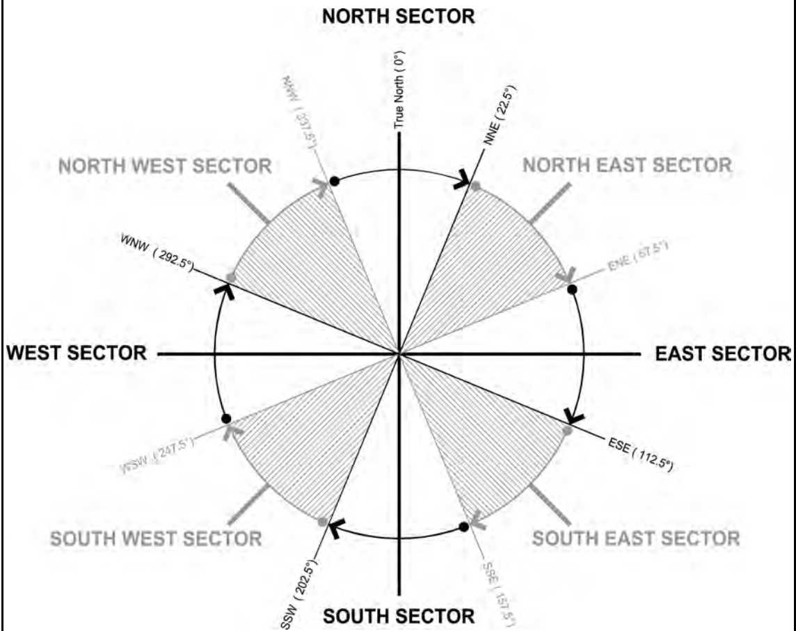
Figure 3.12.2.1 ORIENTATION SECTORS
