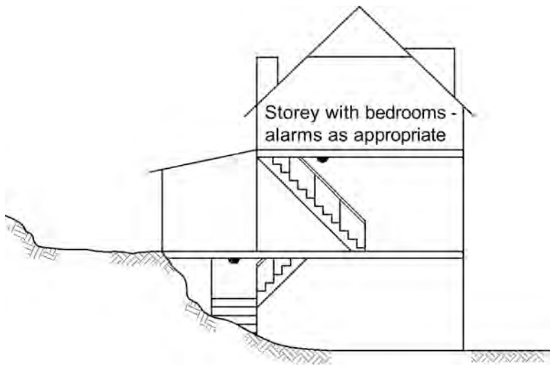
(a) Smoke alarms installed on each storey not containing bedrooms — located in the area of the stairway
