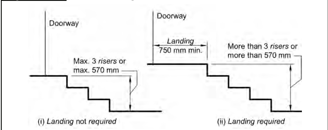
Diagram b. Threshold landing
