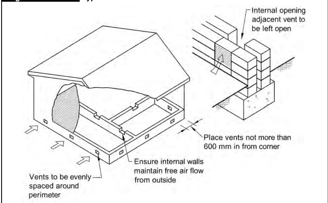
Diagram a. Typical Cross Ventilation of Sub-Floor Area
