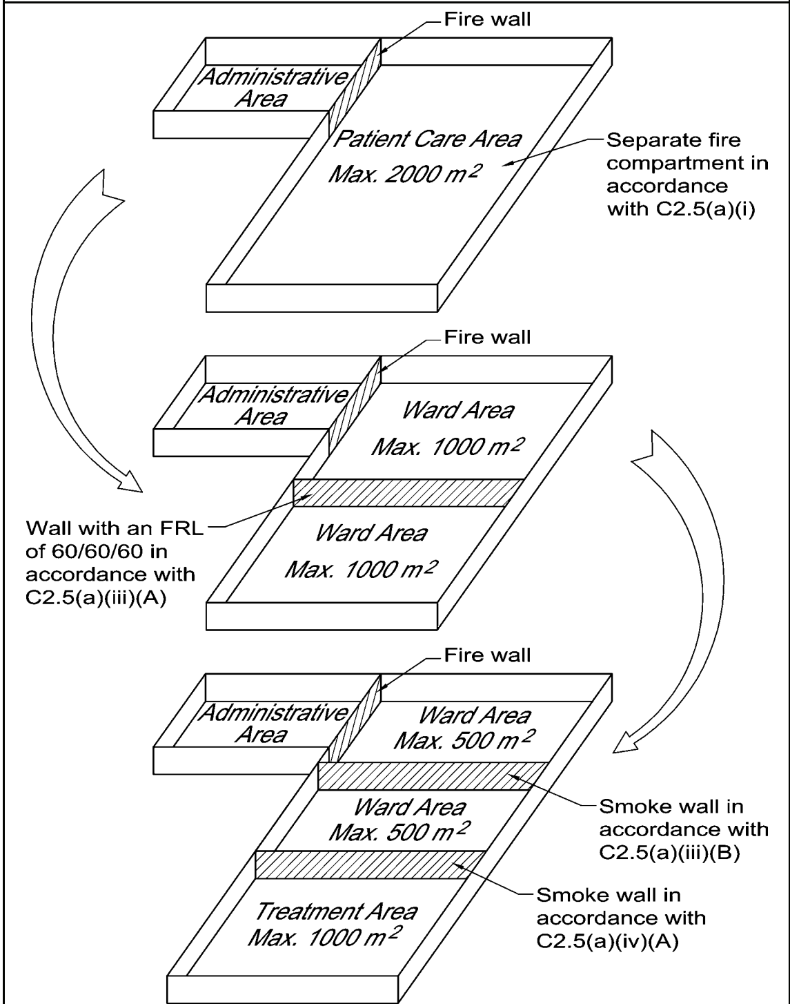
Figure C2.5 PLAN SHOWING ONE METHOD OF COMPLYING WITH C2.5(a) FOR CLASS 9a BUILDINGS
