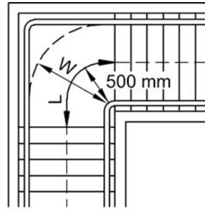
(b) 90° change in direction
