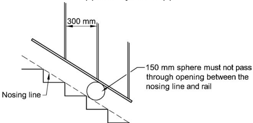
(b) Fire isolated stairways - D2.16(c)
