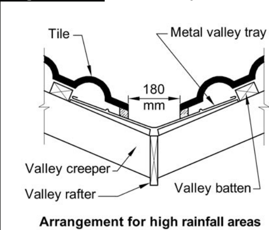
Diagram c. Bedded and pointed valley
