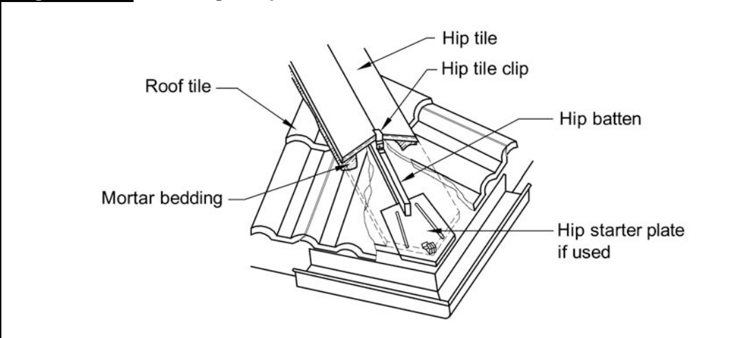
Diagram d. Fastening of hip tiles
