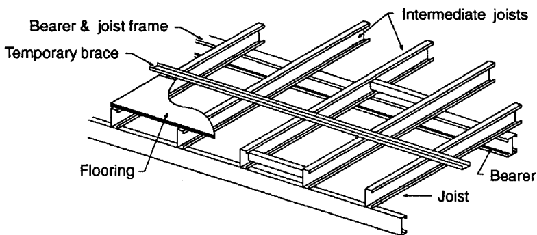
Figure 3.4.2.1 TYPICAL JOIST OVER BEARER FLOORING SYSTEM
