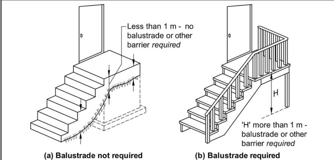
Figure 3.9.2.3 BALUSTRADES OR OTHER BARRIERS — WHEN REQUIRED
