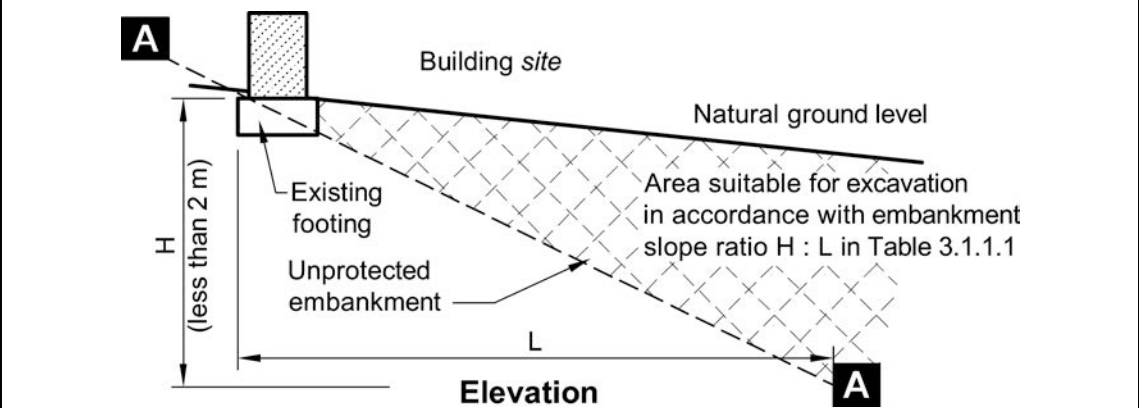
Figure 3.1.1.2 EXCAVATION ADJACENT TO EXISTING BUILDINGS
