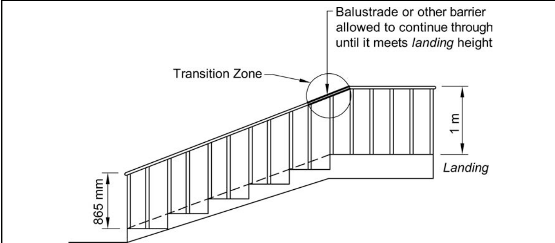
Figure 3.9.2.3 BALUSTRADES OR OTHER BARRIERS — WHEN REQUIRED
