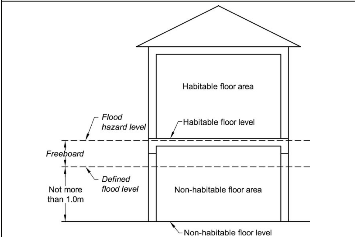
Figure 1.1.5 IDENTIFICATION OF DEFINED FLOOD LEVEL, FLOOD HAZARD LEVEL AND FREEBOARD
