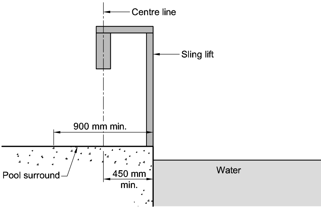
Diagram b. Clear space for sling lift in the transfer position Sectional elevation
