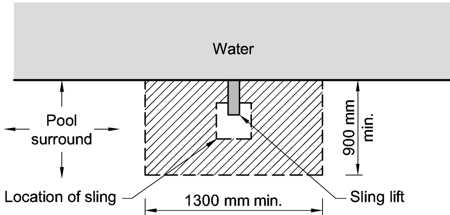
Diagram b. Clear space for sling lift in the transfer position Sectional elevation
