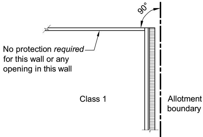
Figure 3.7.1.2a MEASUREMENT OF DISTANCES (Plan view)
