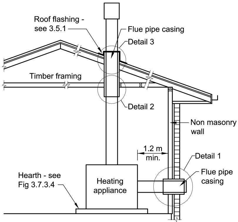
Figure 3.7.3.5 ACCEPTABLE FLUE INSTALLATION DETAILS
