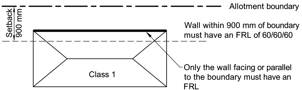
Figure 3.7.1.2a MEASUREMENT OF DISTANCES (Plan view)
