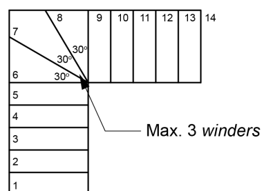
(b) Continuous stairway - 1 flight (90° change in direction)
