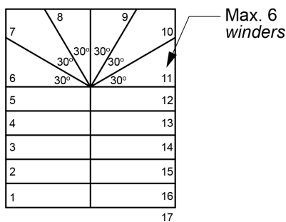
(d) Continuous stairway - 1 flight (180° change in direction)
