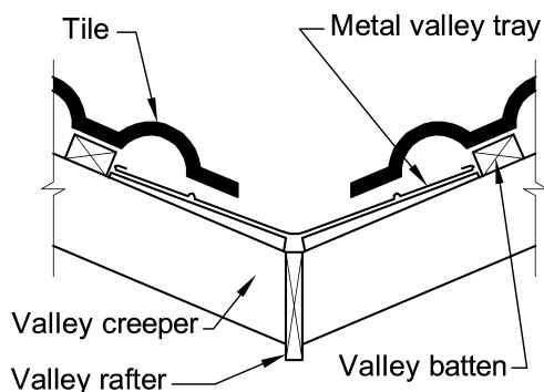
Standard arrangement
