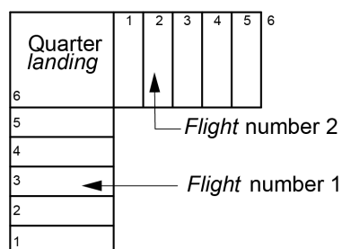
(a) Quarter landing stairway - 2 flights
