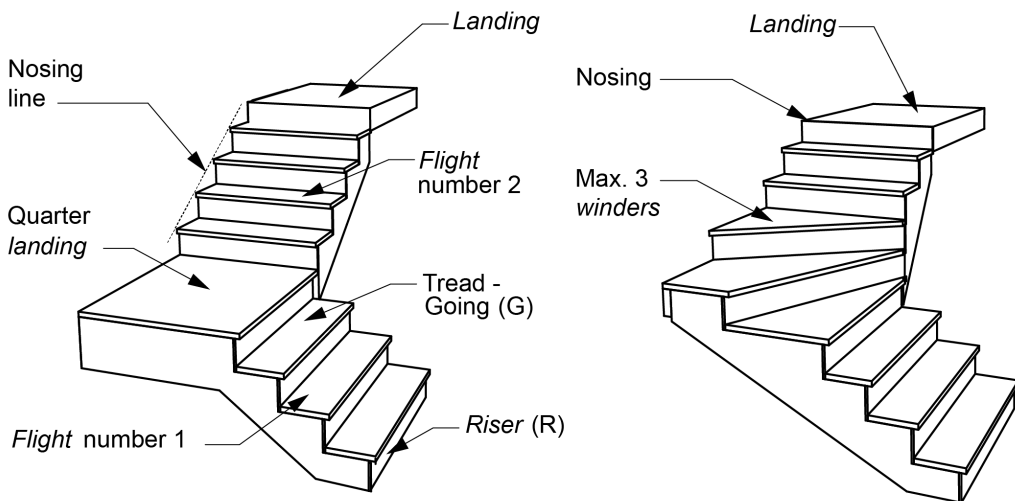
(a) Quarter landing stairway - 2 flights
