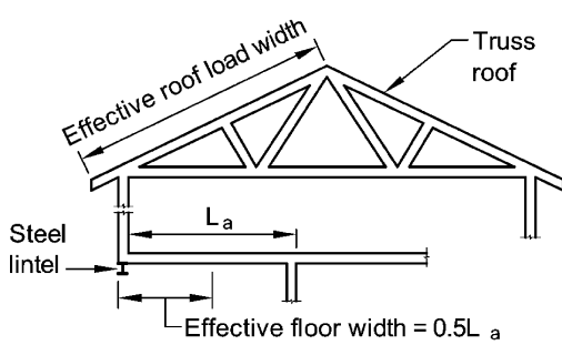
(a) Floor and truss roof
