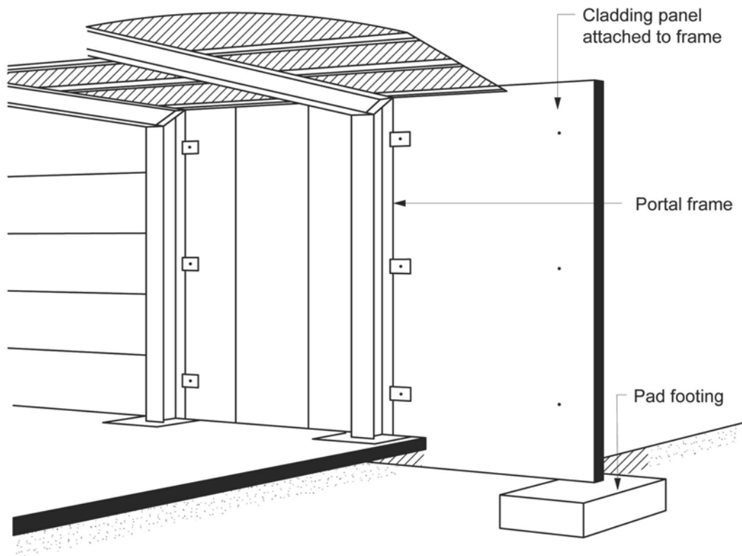
Figure Spec C1.11(1) Typical non-loadbearing panels required to comply with Specification C1.11 (Panels may be full bay, multiple vertically or horizontally spanning)
