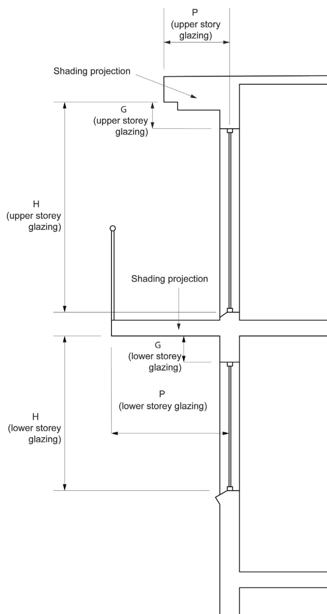
Figure 7 Permanent external shading - Measurement of P, G and H
